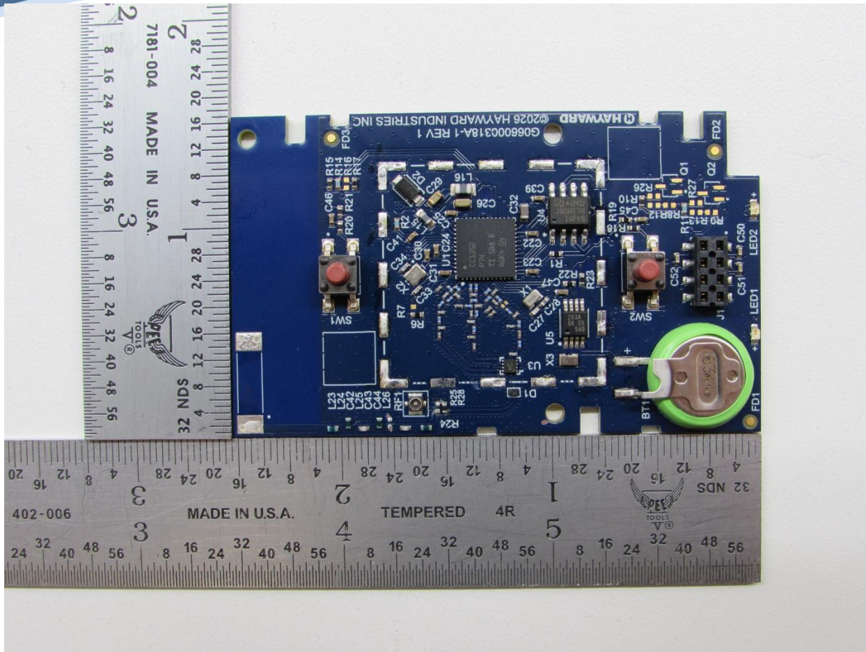
External antenna cover off
