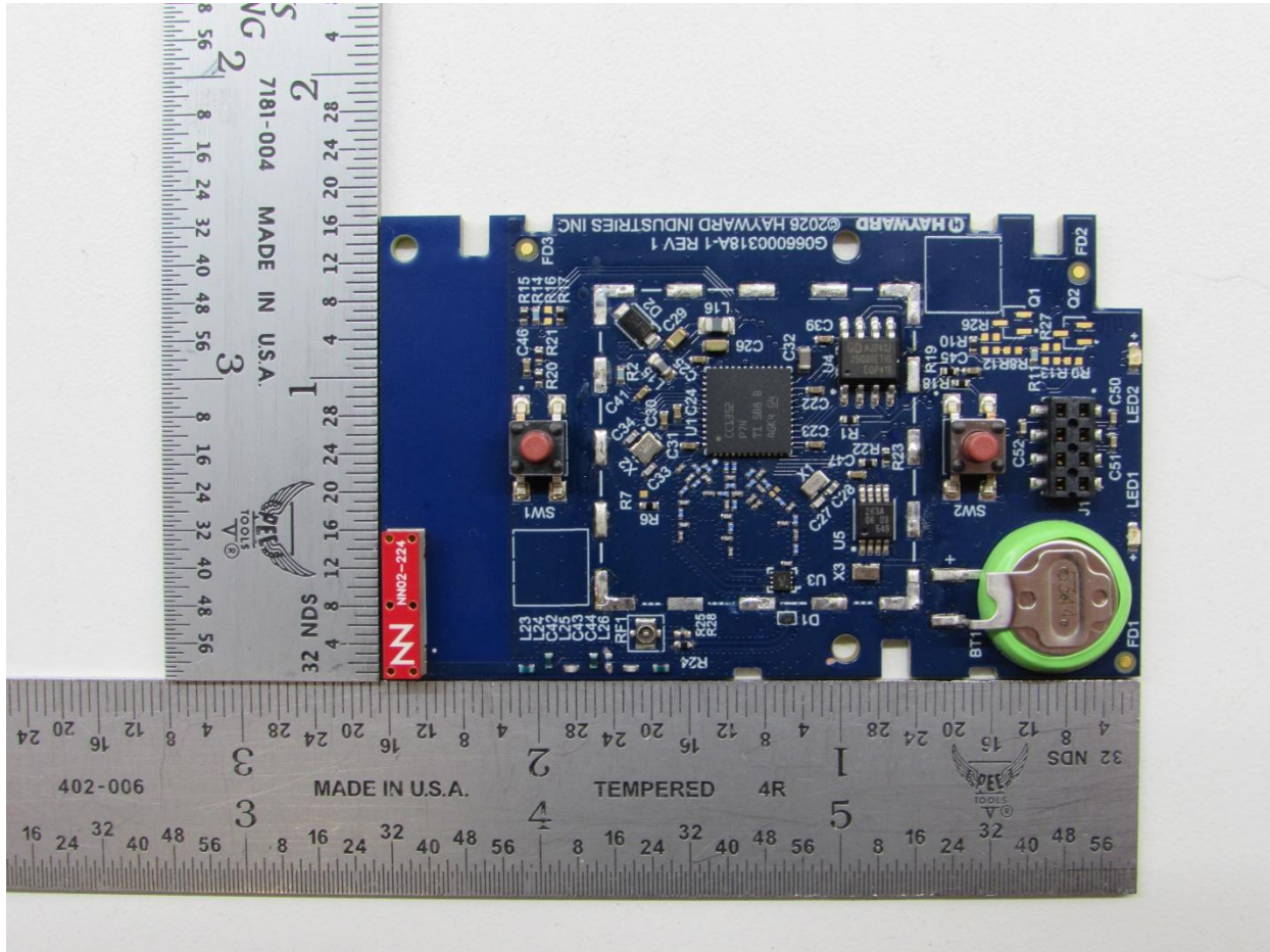
Chip antenna cover off
