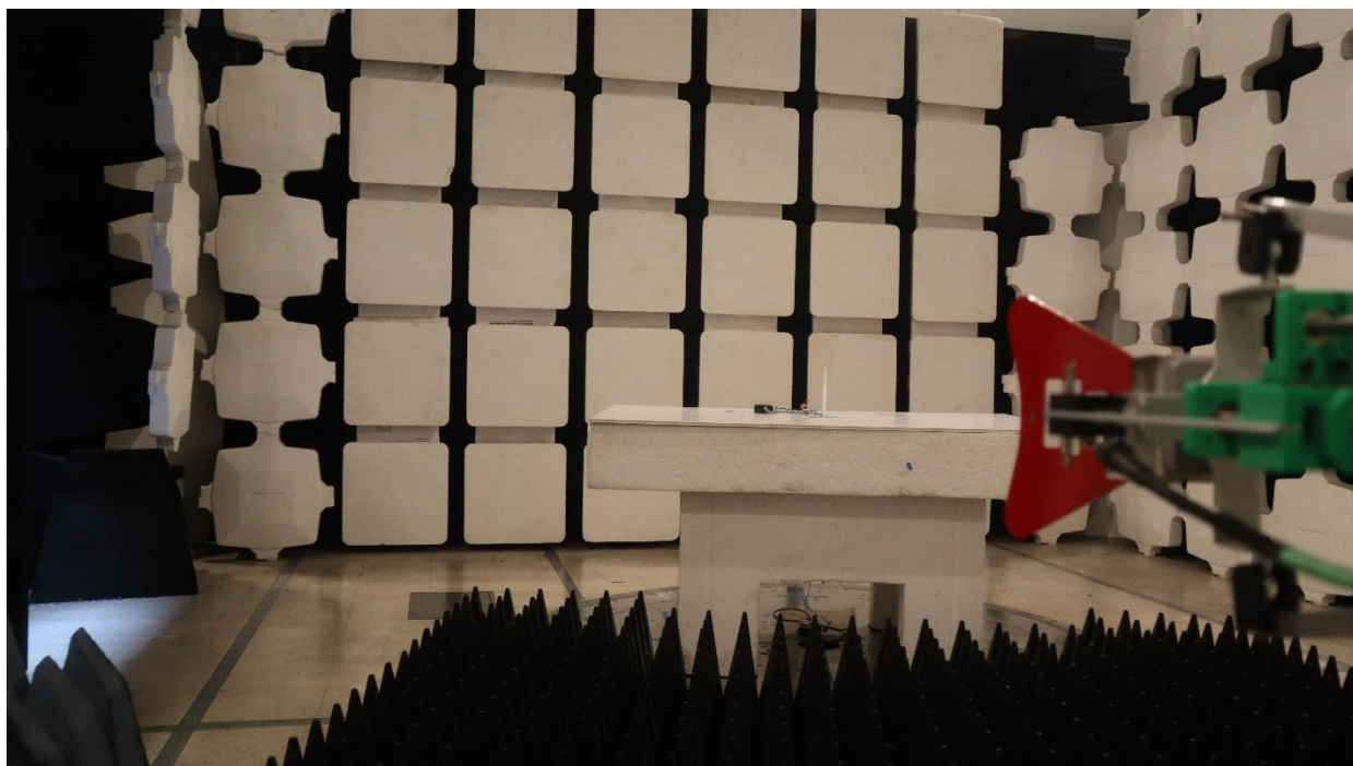
1-18GHz Digital Emissions - External Antenna
