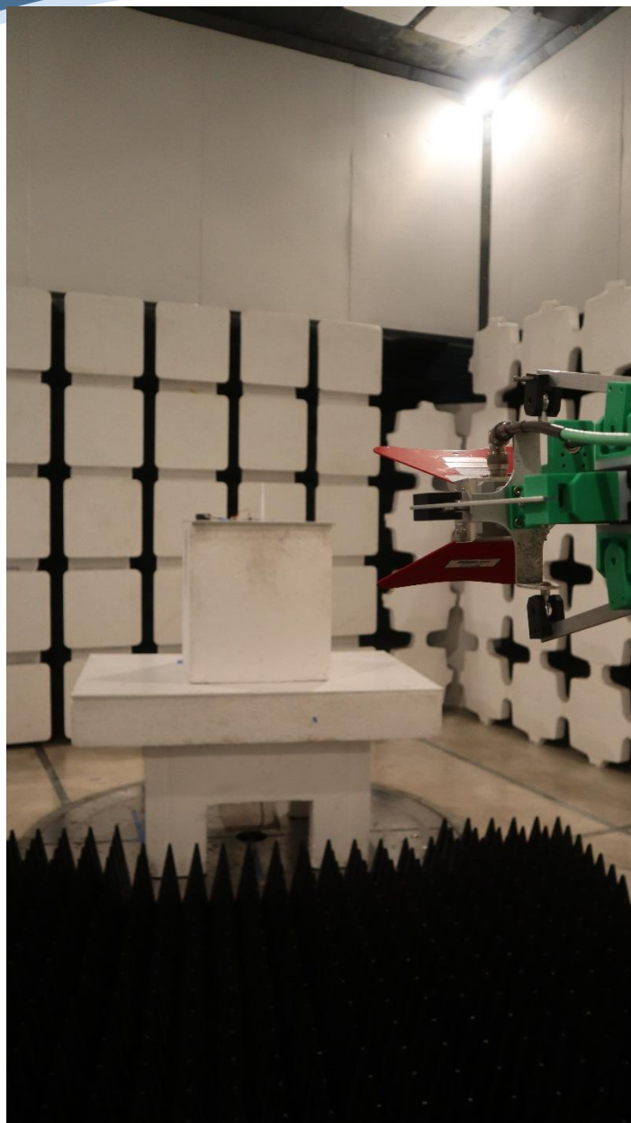
Tx Spurious 1-18GHz – External Antenna
