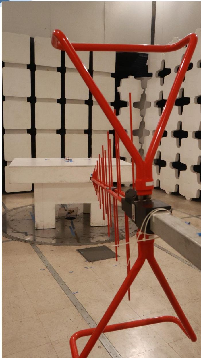
Tx Spurious 30MHz-1GHz – Internal Antenna
