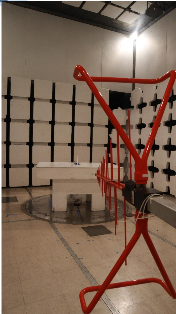
Tx Spurious 30MHz-1GHz – External Antenna
