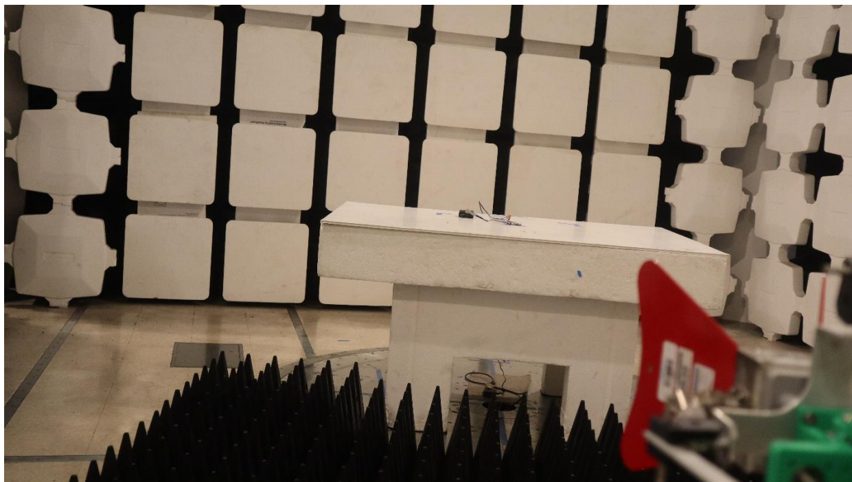
1-18GHz Digital Emissions – Internal Antenna
