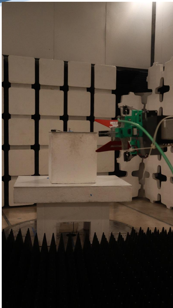
Tx Spurious Emissions 1-18GHz – Internal Antenna
