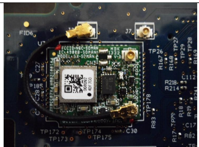
Host PCBA with EUT Close up View
