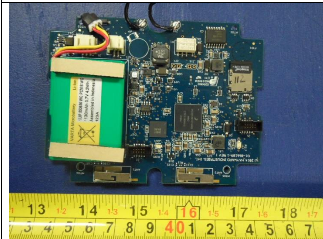
Host – PCBA Main Board Top View
