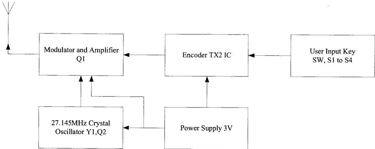
The Block Diagram Of Transmitting Circuit For 27.145MHz
