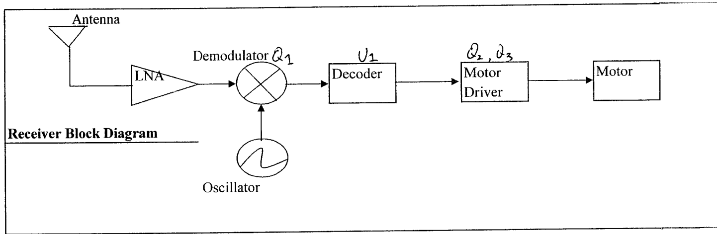
Receiver Block Diagram
