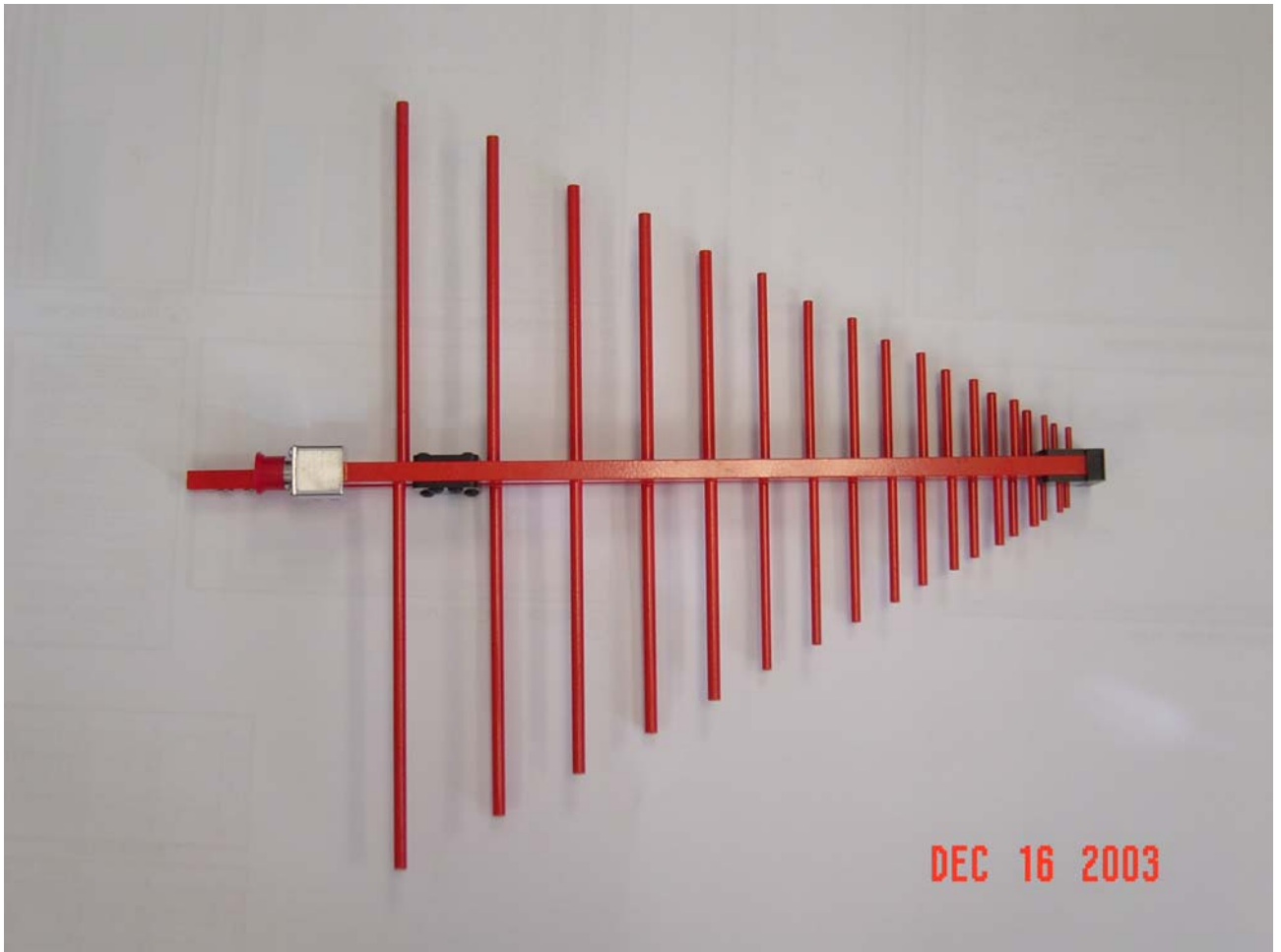
Standard LPA antenna, internal view:
