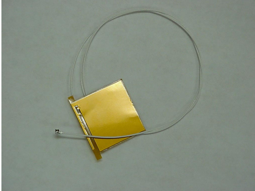
Inverted F
