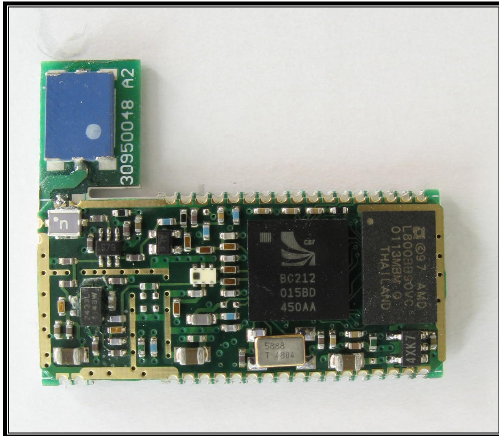
Photograph 10: BT Module Right Angle Version without Shield – Front View
