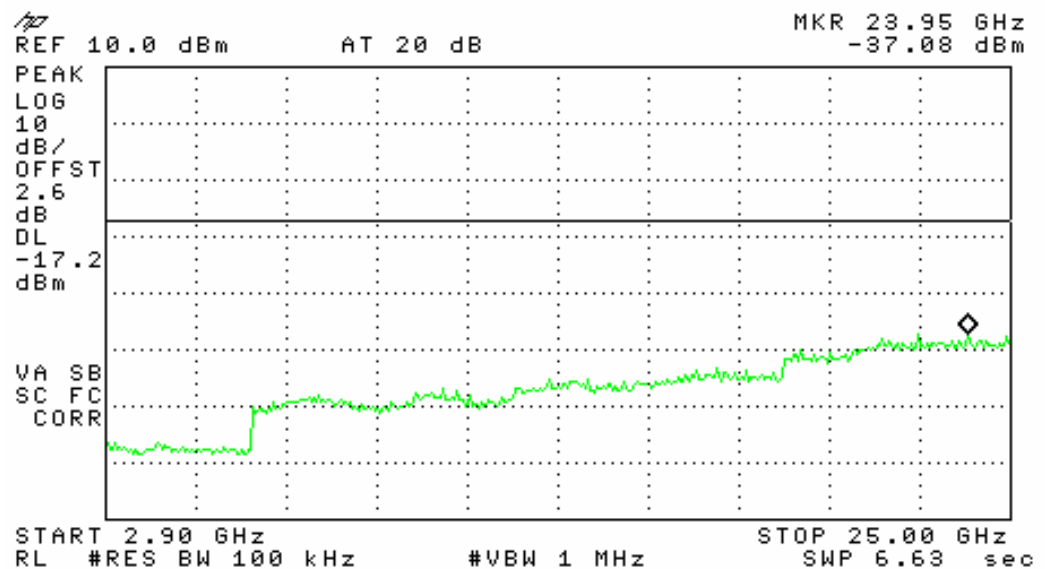
Plot #4: MIDDLE Channel (2441 MHz) Spurious Emission 2.9 – 25 GHz
