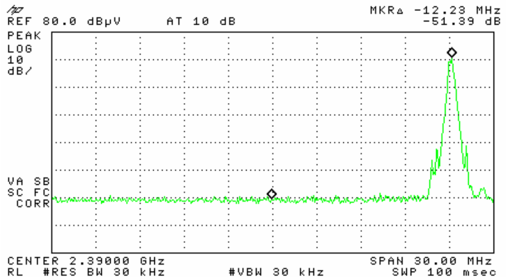
Plot #1: Delta between 2402 MHz (LOW channel) and 2390 MHz
