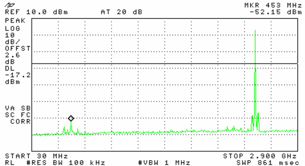
Pot #3: MIDDLE Channel (2441 MHz) Spurious Emission 30 MHz - 2.9 GHz
