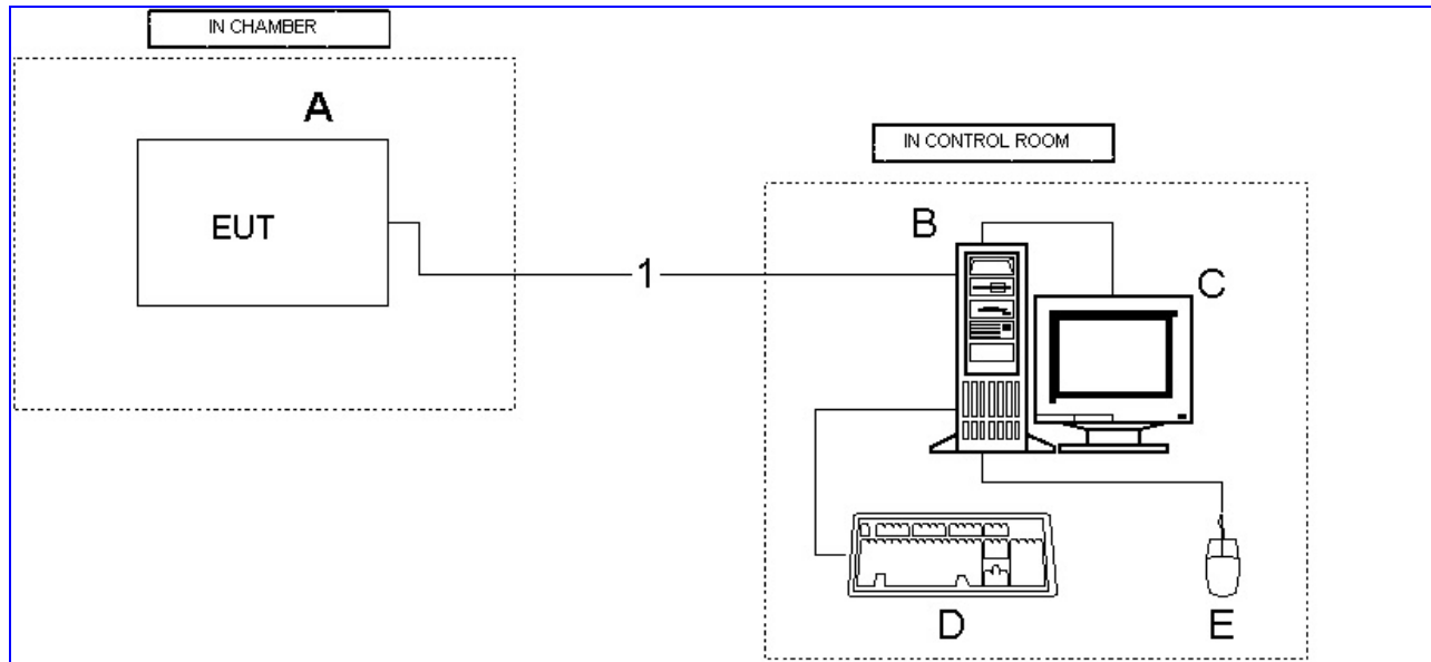
Figure 1. Block Diagram of CEV and REE Test Configuration
