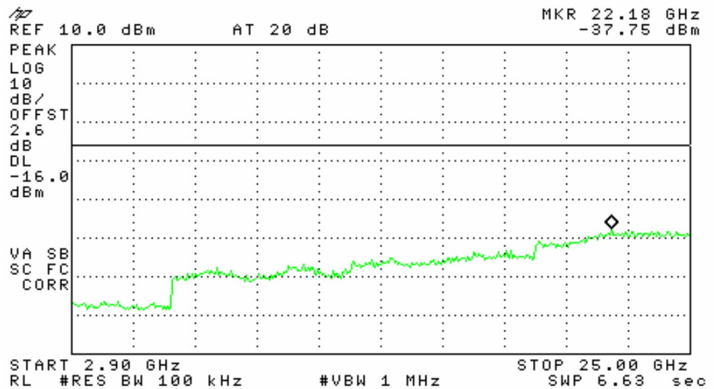
Plot #2: LOW Channel (2402 MHz) Spurious Emission 2.9 – 25 GHz
