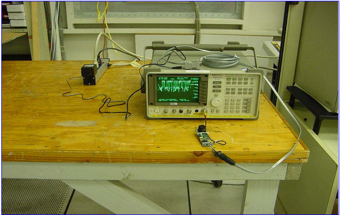
Photograph 3. RF Antenna Conducted, Test Setup
