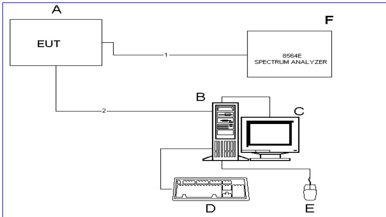
Figure 2. RF Antenna Conducted Test Configuration
