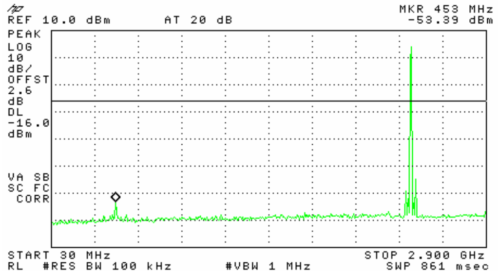
Plot #1: LOW channel (2402 MHz) Spurious Emission 30 MHz - 2.9 GHz
