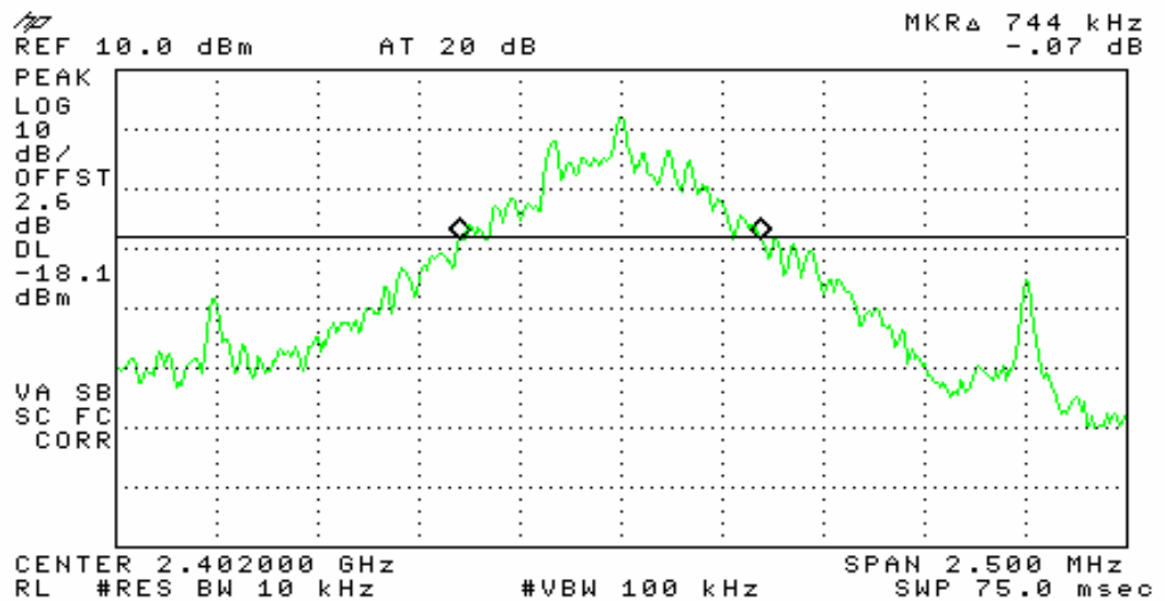
Plot #1: LOW Occupied BW = Low Channel
