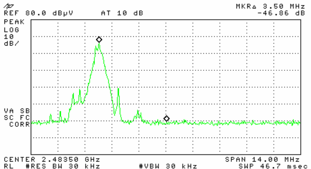
Plot #2: Delta between 2480 MHz (HIGH channel) and 2483.5 MHz
