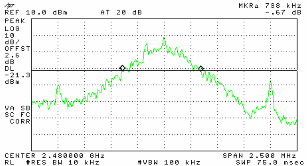
Plot #3: HI occupied BW = High Channel
