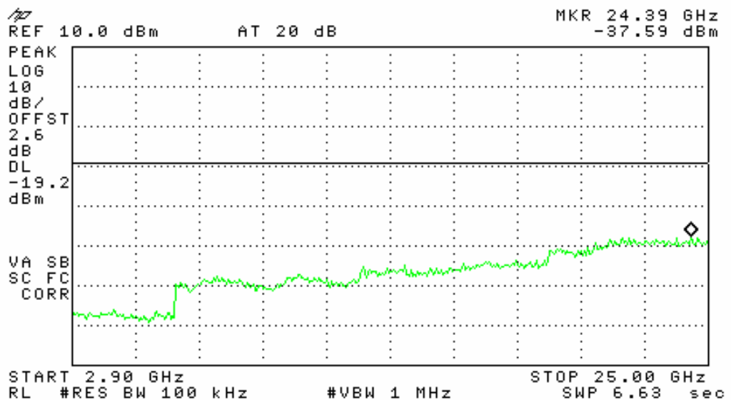
Plot #6: HIGH Channel (2480 MHz) Spurious Emission 2.9 – 25 GHz
