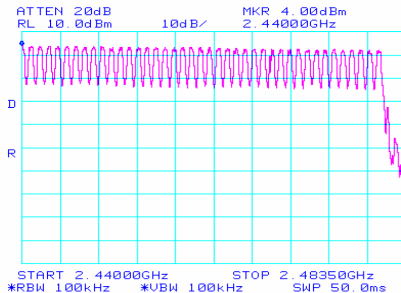
Plot #2: 2 nd half = Top half of Frequency Range
