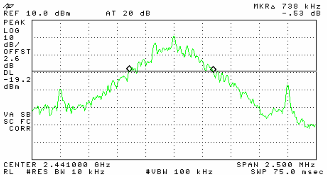
Plot #2: MID Occupied BW = Middle Channel
