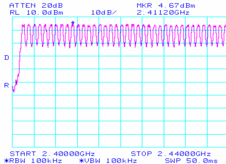
Plot #1: 1 st half = Bottom half of Frequency Range
