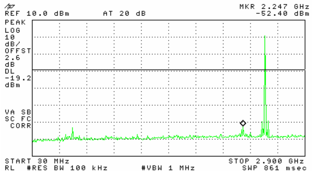
Plot #5: HIGH Channel (2480 MHz) Spurious Emission 30 MHz - 2.9 GHz
