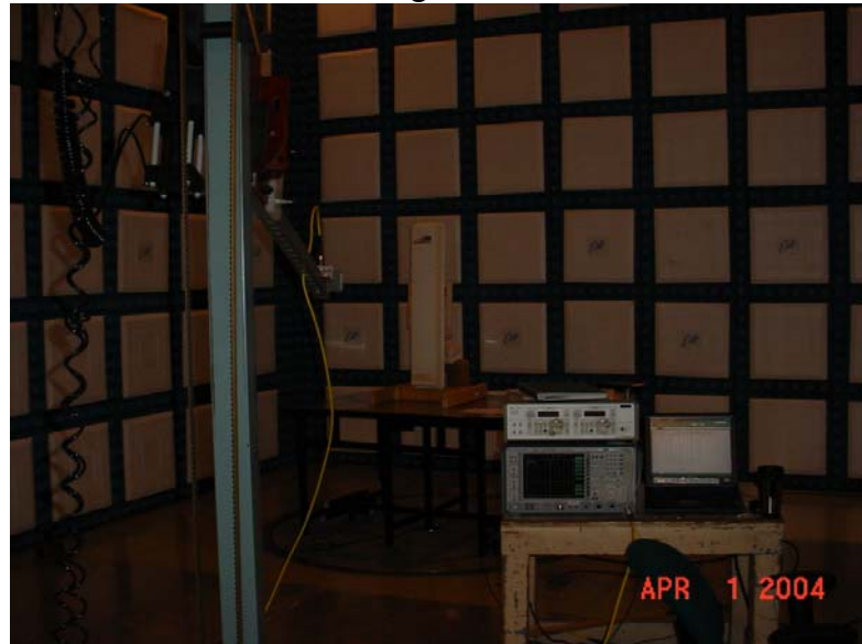
Test Setup for Measurement of Radiated Emissions from a RadioWaves 90° Sectored Antenna
