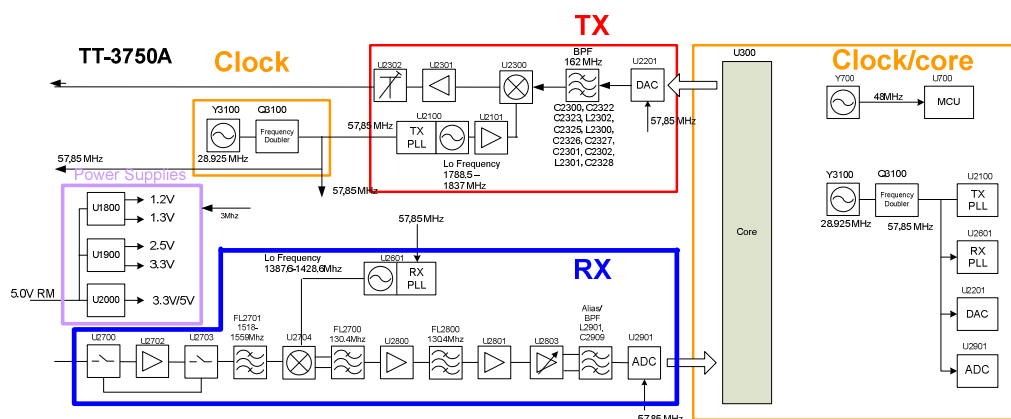
Figure 10 Radio module block diagram function by colour
