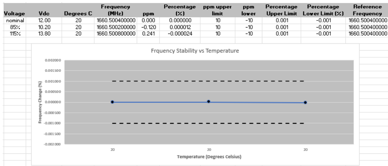
Figure 2.6.6-6: Frequency Stability at Extreme Voltages – High Channel
