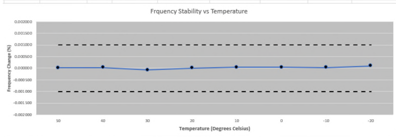
Figure 2.6.6-5: Frequency Stability at Various Temperatures – High Channel
