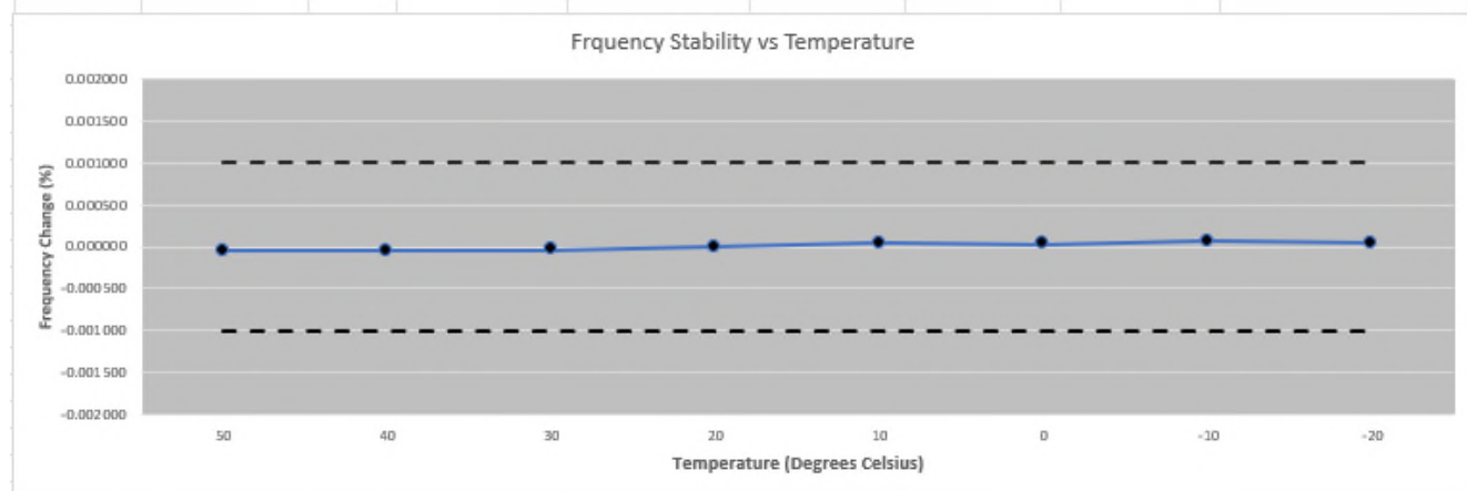
Figure 2.6.6-3: Frequency Stability at Various Temperatures – Mid Channel
