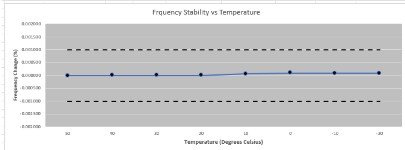
Figure 2.6.6-1: Frequency Stability at Various Temperatures – Low Channel
