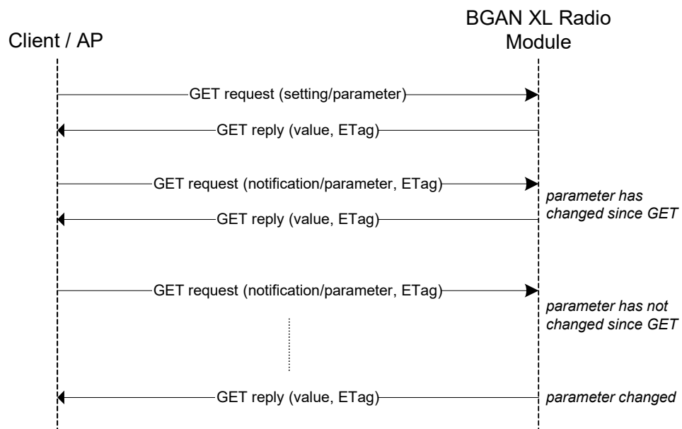
Figure 7-3: Notification sequence
