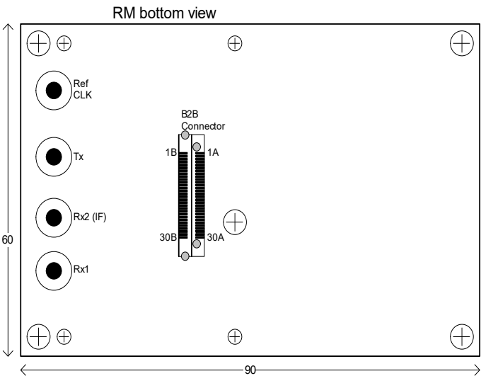
Figure 5-7: Connectors of the BGAN XL Radio Module
