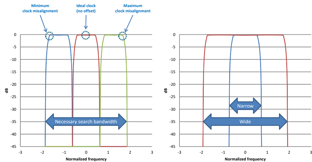
Figure 8-24: Wide and narrow filter characteristics.
