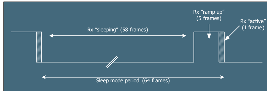
Figure 11-6: SDM sleep mode sequence (example).
