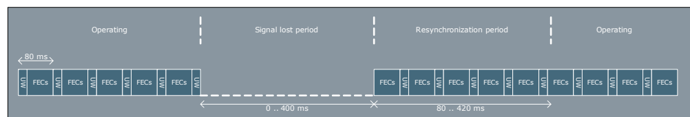
Figure 11-8: Modem re-synchronization.
