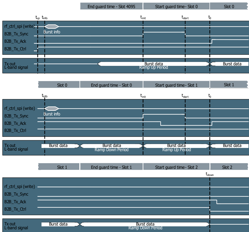
Figure 9-19: RF control interface signals during a two-burst sequence
