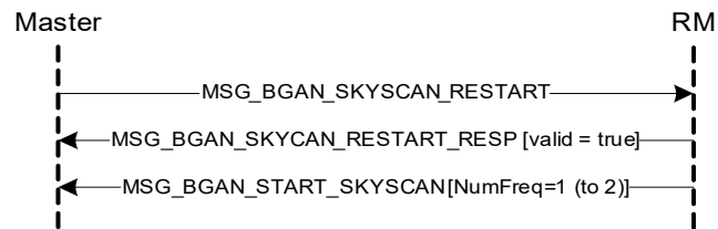
Figure 8-26: Restart of the satellite search
