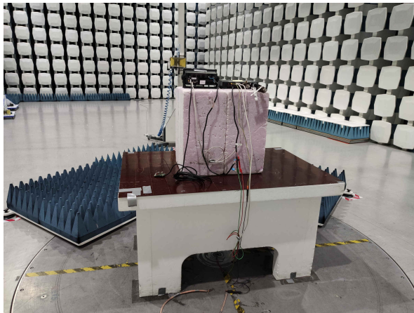
Radiated Emissions 1 – 2 GHz
