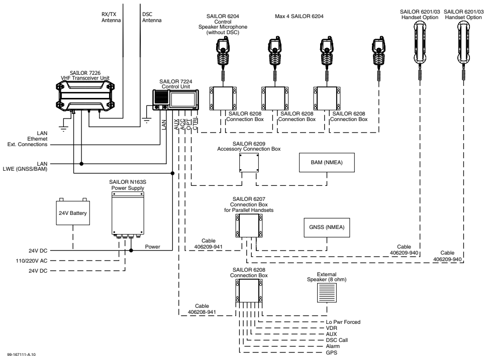
Figure 2: System configuration, example
