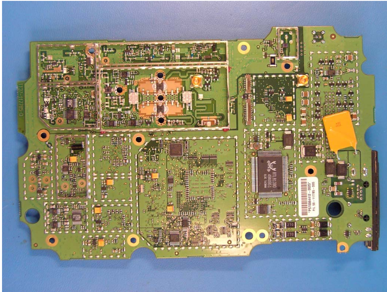
Figure 5 Mainboard
