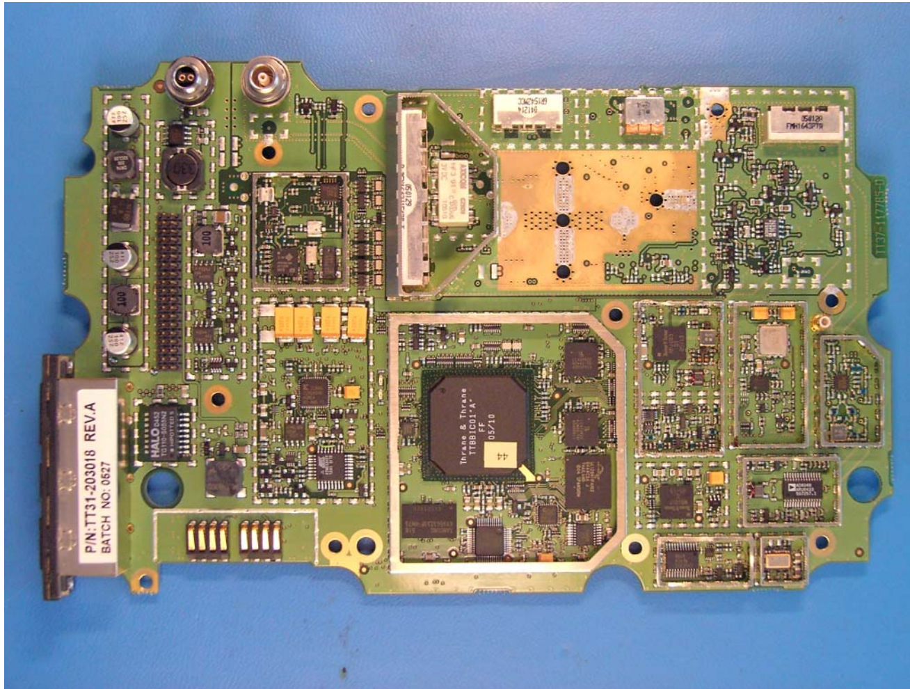
Figure 4 Mainboard
