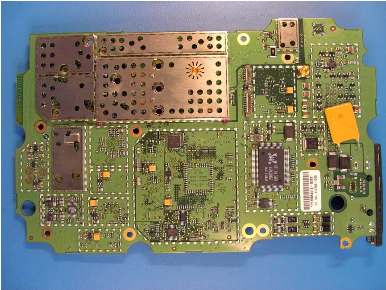
Figure 3 Mainboard
