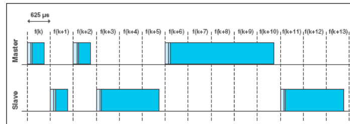
Figure 2.1: Multi-slot packets
