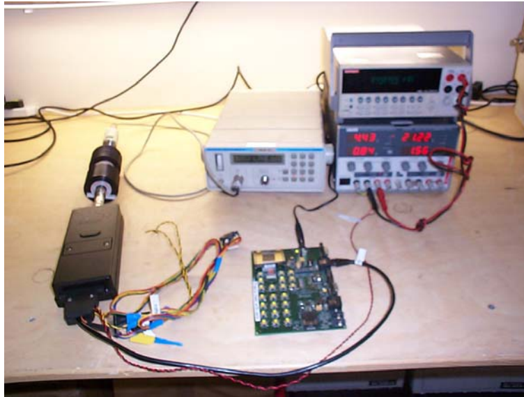
PHOTOGRAPH 2. CONDUCTED TEST SETUP
