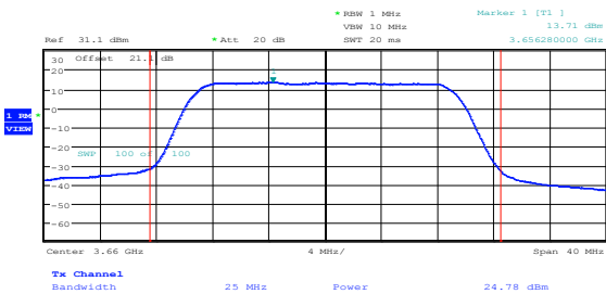
Figure 8.3-1: Peak output power and PSD sample plot at cho with QPSK
