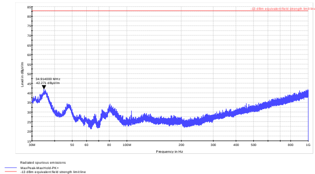
Figure 8.5-21: Spurious radiated emissions sample plot 30–1000 MHz, Hub
