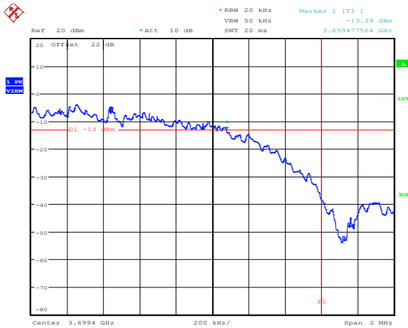
Figure 8.2-2: Lower cross point ( f_L ) sample plot for 256-QAM
