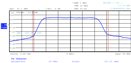
Figure 8.3-3: Peak output power and PSD sample plot at ch1 with QPSK
