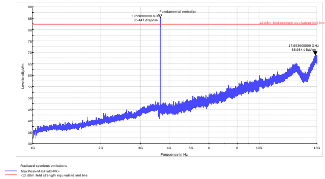
Figure 8.5-23: Spurious radiated emissions sample plot 1–18 GHz, Hub
