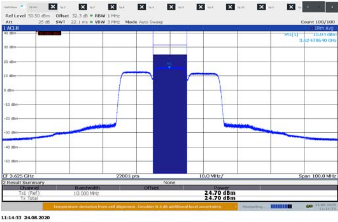
Figure 8.1-6: Ouput power dBm/10 MHz sample plot,3cc 10 MHz channel
