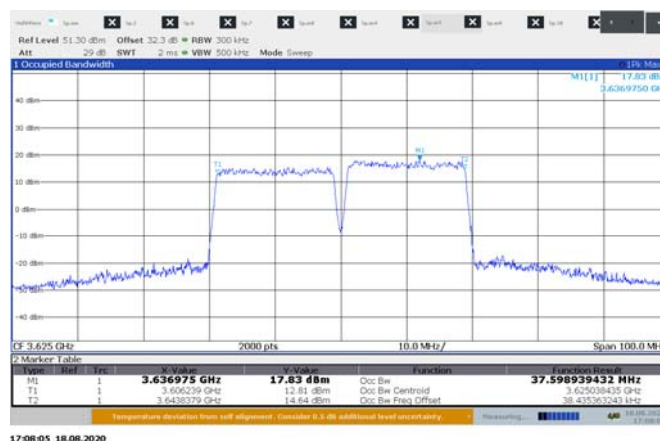
Figure 8.3-2: Occupied bandwidth sample plot for 2CC 20 MHz channel
