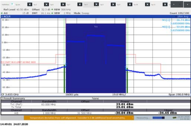
Figure 8.4-26: Emission measurement within 0-10 MHz from the SAS assigned channel edge, sample plot for 20 MHz 3cc additional high channel
