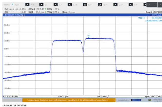
Figure 8.1-11: PSD dBm/1 MHz sample plot,2cc 20 MHz channel
