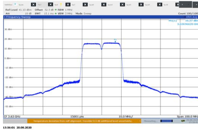
Figure 8.1-9: PSD dBm/ 1 MHz sample plot,2cc 10 MHz channel
