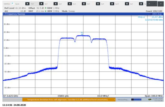
Figure 8.1-10: PSD dBm/1 MHz sample plot,3cc 10 MHz channel
