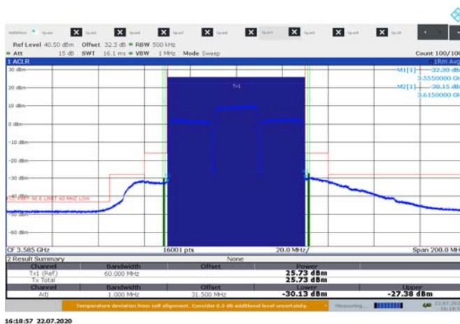
Figure 8.4-20: Emission measurement within 0-10 MHz from the SAS assigned channel edge, sample plot for 20 MHz 3cc low channel
