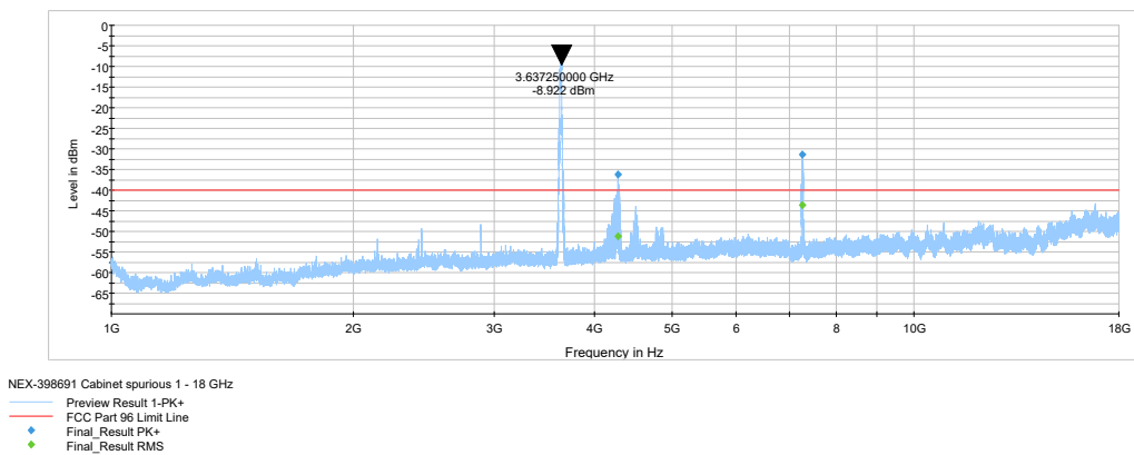
Figure 8.5-2: Cabinet spurious emissions sample plot (1 to 18 GHz)
