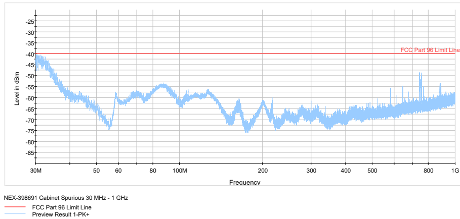
Figure 8.5-1: Cabinet spurious emissions sample plot (30 to 1000 MHz)
