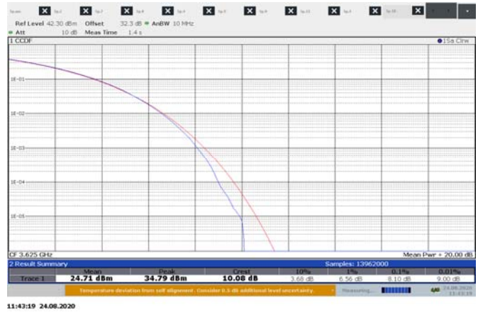
Figure 8.2-2: CCDF sample plot, 3cc 10 MHz channel
