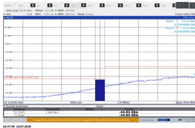
Figure 8.5-19: Low Banedge for 20 MHz 3cc channel at 3530 MHz sample plot
