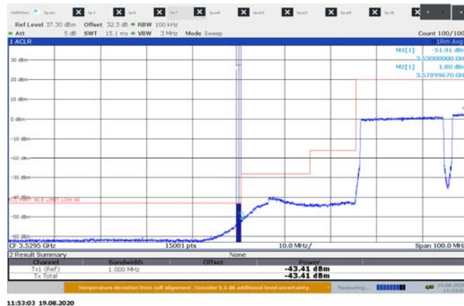
Figure 8.5-14: Low Bandedge for 20 MHz 2cc channel at 3530 MHz sample plot
