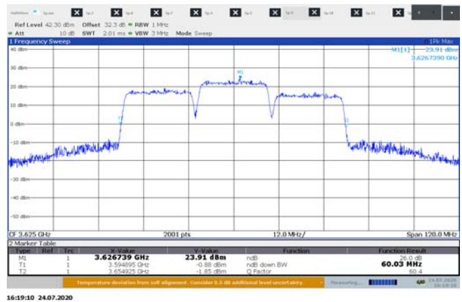
Figure 8.3-8: 26 dB bandwidth sample plot for 3 CC 20 MHz channel
