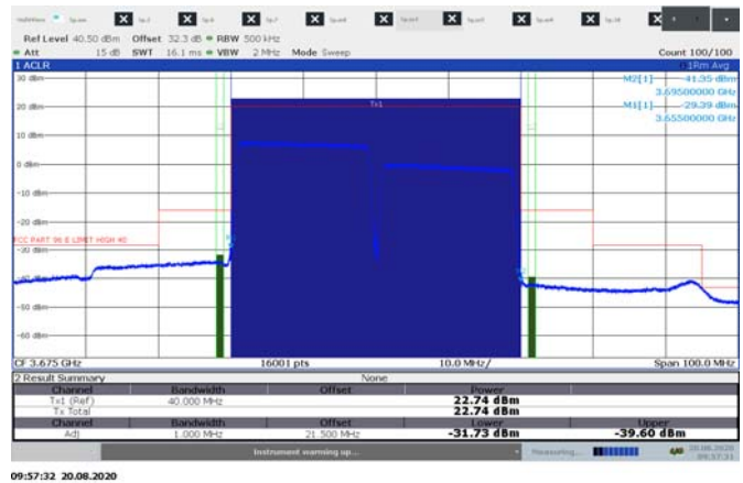
Figure 8.4-18: Emission measurement within 0-10 MHz from the SAS assigned channel edge, sample plot for 20 MHz 2cc high channel
