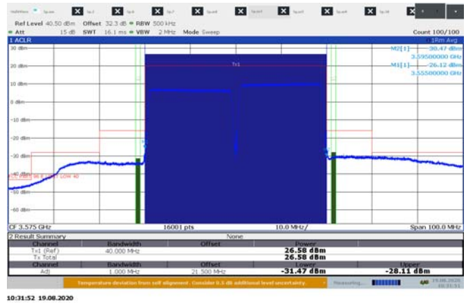
Figure 8.4-14: Emission measurement within 0-10 MHz from the SAS assigned channel edge, sample plot for 20 MHz 2cc low channel
