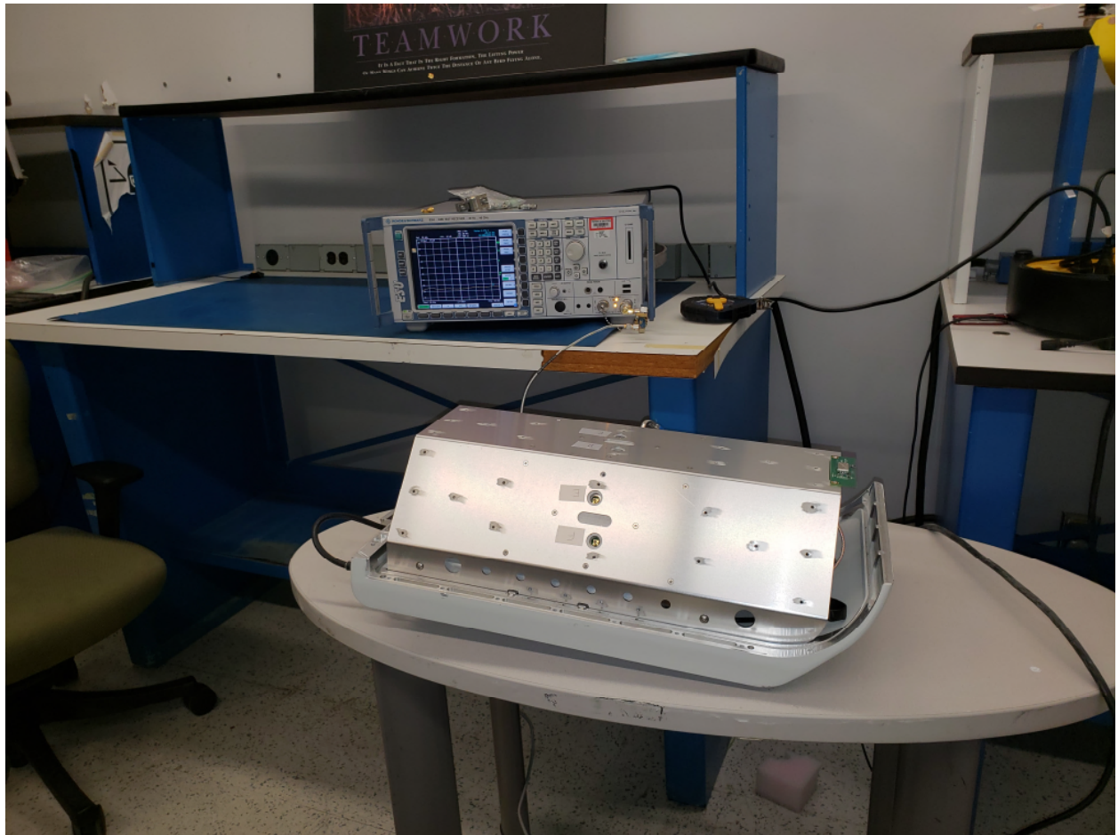
Antenna port conducted emissions
