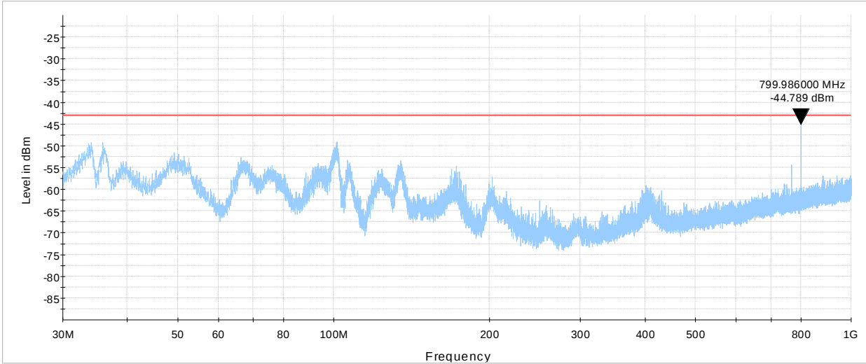
NEX-391430 Radiated emissions 30 MHz - 1 GHz
