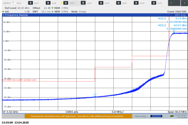
Figure 8.5-4: Low Bandedge for 10 MHz channel at 3530 MHz sample plot
