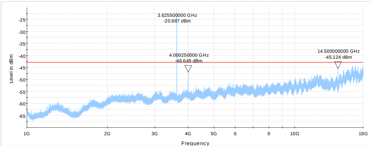
NEX-391430 Cabinet Spurious 1 - 18 GHz
