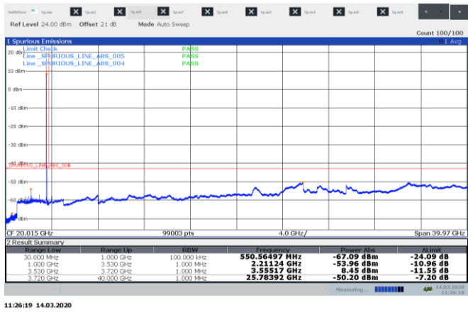
Figure 8.5-1 : Conducted spurious emissions for 10 MHz low channel sample plot 30 MHz – 40 GHz
