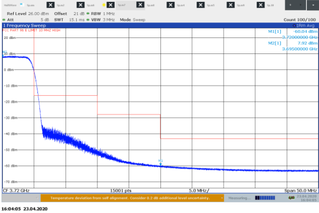
Figure 8.5-5: High Bandedge for 10 MHz channel at 3720 MHz sample plot
