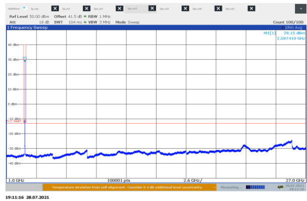
Figure 8.2-22: Conducted spurious emissions 1 - 27 GHz at 15 MHz mid channel ,sample plot
