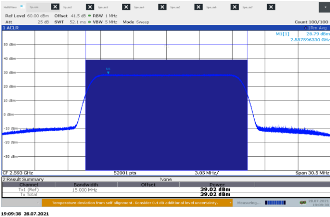
Figure 8.1-2: Output power for 15 MHz channel BW, sample plot
