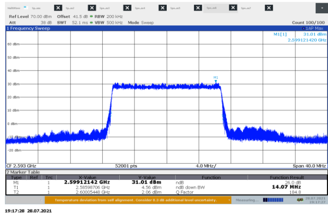
Figure 8.3-2: 26 dB sample plot for 15 MHz channel
