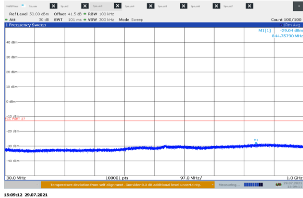
Figure 8.2-9: Conducted spurious emissions 30 MHz -1 GHz at 5 MHz low channel ,sample plot
