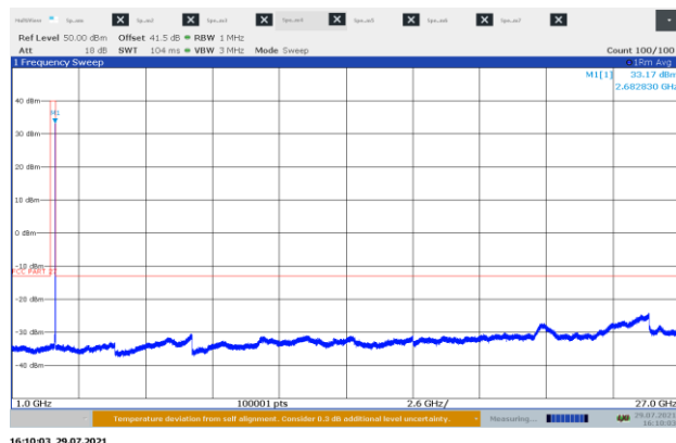
Figure 8.2-18: Conducted spurious emissions 1 - 27 GHz at 5 MHz high 2684 MHz channel, sample plot
