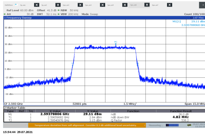
Figure 8.3-1: 26 dB sample plot for 5 MHz channel
