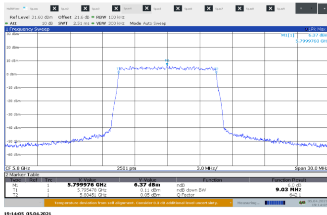
Figure 8.5-3: 6 dB bandwidth 10 MHz, sample plot
