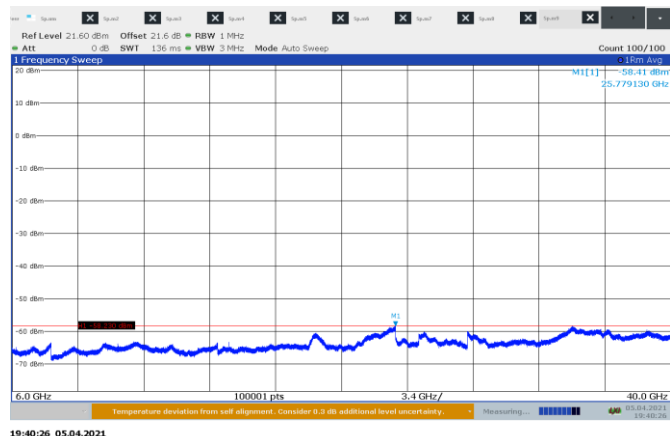
Figure 8.8-4: Conducted average spurious emissions 6- 40 GHz on low channel 10 MHz sample plot
