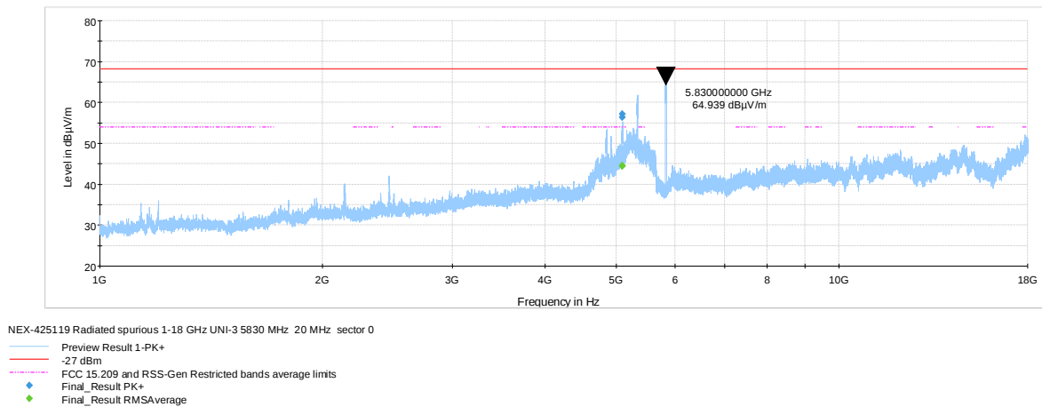
Figure 8.8-44: Radiated spurious emissions 1 - 18 GHz, 5830 MHz Channel
