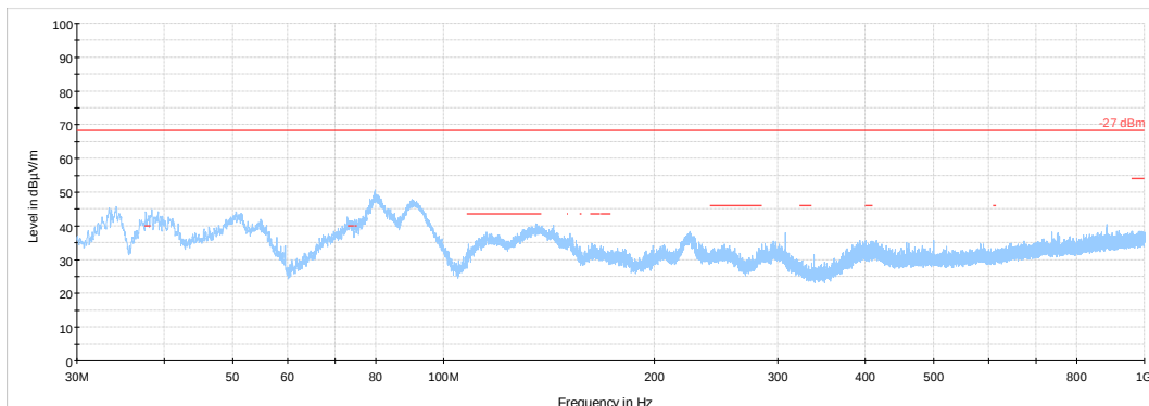
Figure 8.8-38: Radiated spurious emissions 30 MHz – 1 GHz, Low Channel
