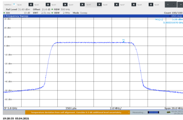
Figure 8.7-3: Sample plot for PSD on 10 MHz
