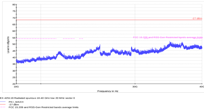
Figure 8.8-46: Radiated spurious emissions 18 - 40 GHz, low Channel
