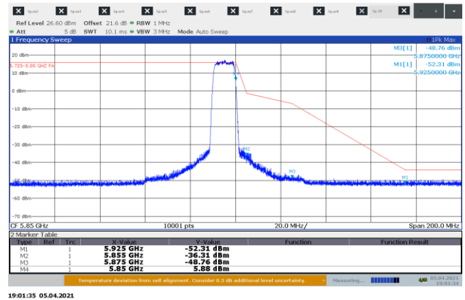
Figure 8.8-14: Conducted Banedge mask on high channel 10 MHz channel sample plot
