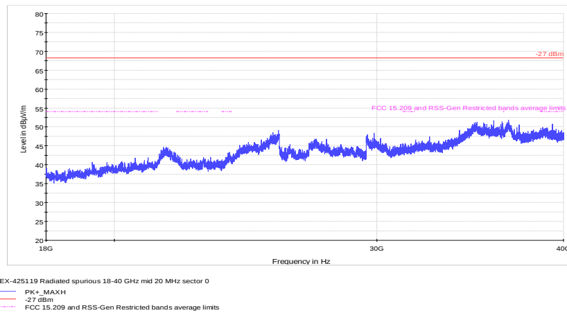
Figure 8.8-47: Radiated spurious emissions 18 – 40 GHz, mid Channel
