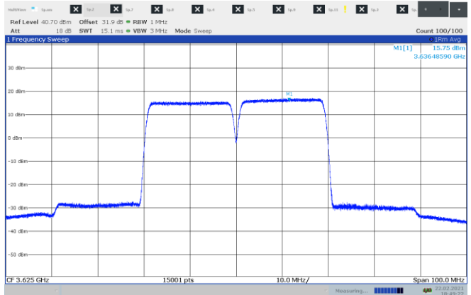
Figure 8.1-6: Output power sample plot, 2cc 20 MHz channel
