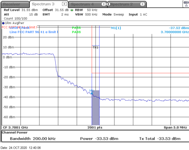
Figure 8.4-10: Emission measurement within 0-1 MHz high end from the SAS assigned channel edge, sample plot for 1CC 20 MHz channel
