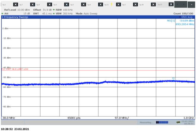
Figure 8.5-9: Conducted spurious emissions for 2CC 20 MHz channel sample plot 30 MHz – 1GHz
