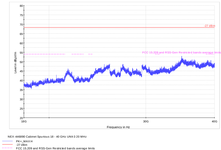
Figure 8.8-42: Cabinet spurious emissions 18 - 40 GHz, 20 MHz Channel
