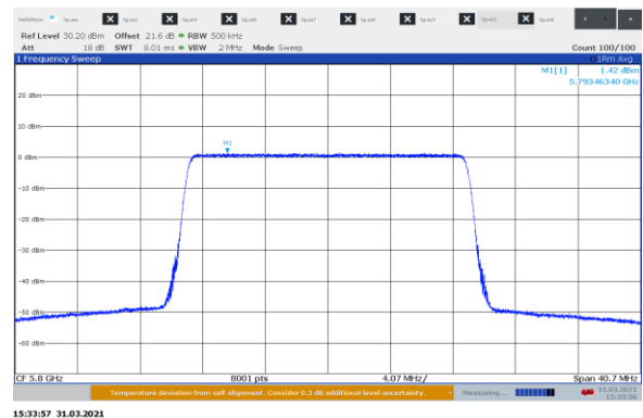
Figure 8.7-8: Sample plot for PPSP on 20 MHz
