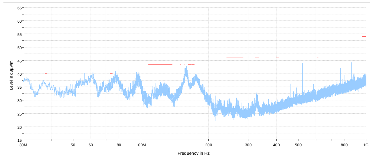
Figure 8.8-37: Cabinet spurious emissions 30 MHz – 1 GHz, 10 MHz Channel
