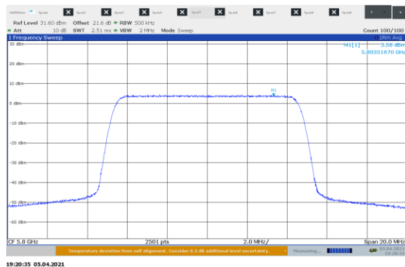
Figure 8.7-7: Sample plot for PPSP on 10 MHz
