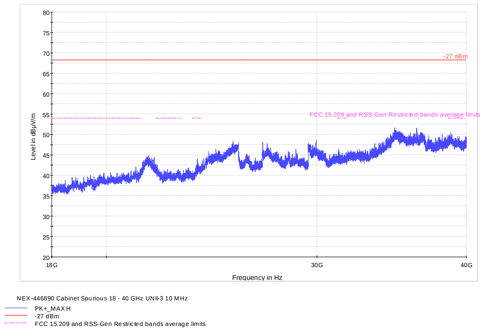
Figure 8.8-41: Cabinet spurious emissions 18 - 40 GHz, 10 MHz Channel
