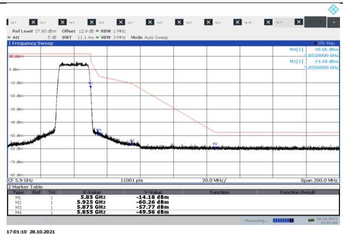
Figure 8.8-32: Conducted Banedge mask on high channel 20 MHz channel sample plot
