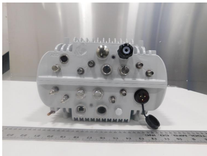
Figure 9.1-6: Bottom view photo
