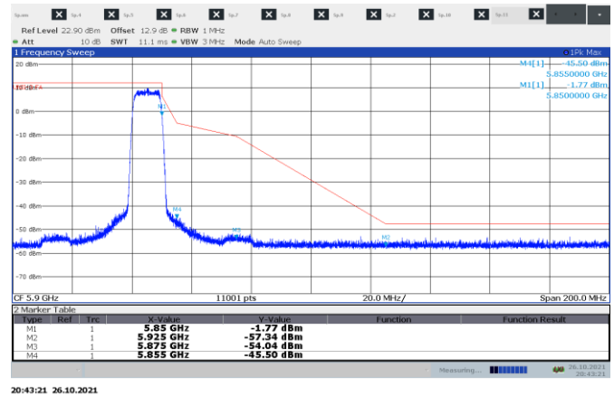
Figure 8.8-14: Conducted Banededge mask on high channel 10 MHz channel sample plot
