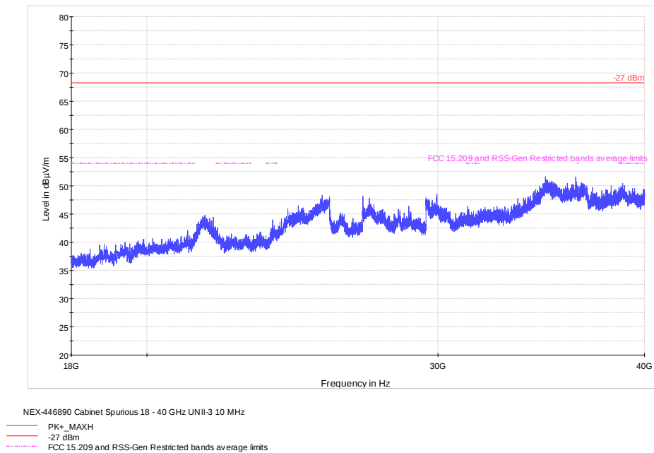
Figure 8.8-41: Cabinet spurious emissions 18 - 40 GHz, 10 MHz Channel
