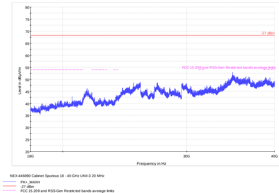
Figure 8.8-42: Cabinet spurious emissions 18 - 40 GHz, 20 MHz Channel
