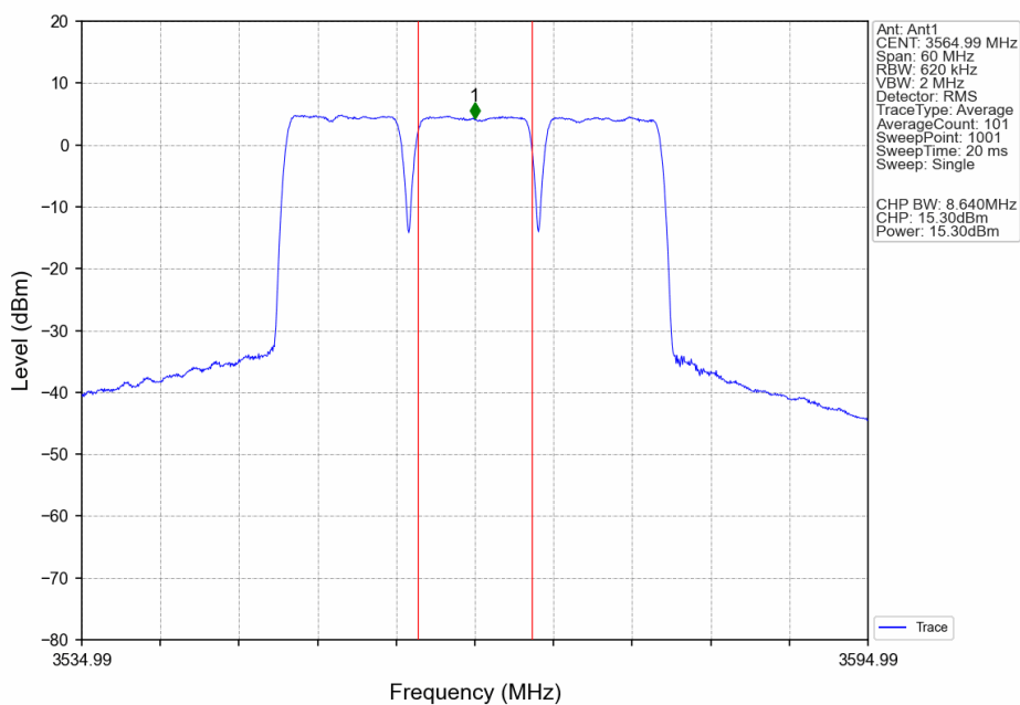
n78d_BS Type 1-C_30_Continuous_NTNV_CC1:10 CC2:10 CC3:10MHz_NR-FR1-TM3.1a_CC1:3555 CC2:3564.99 CC3:3574.98MHz Ant1
