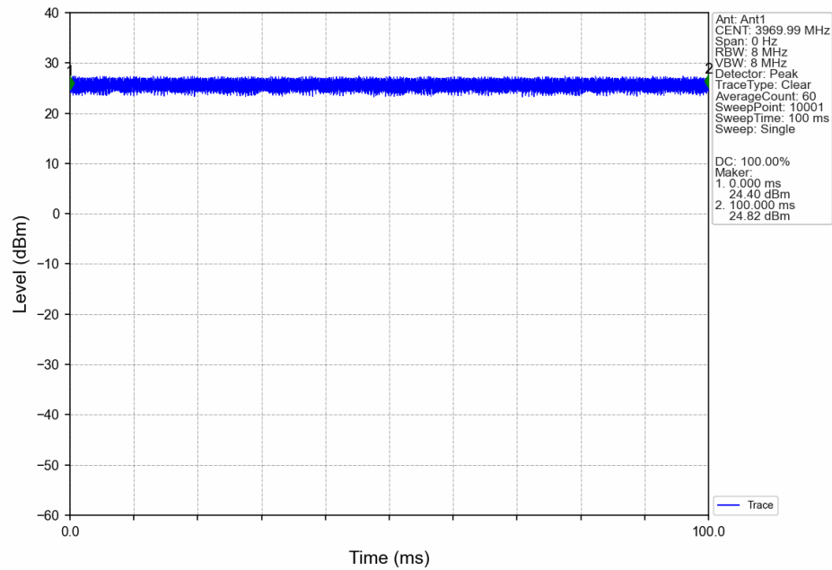
n77a_BS Type 1-C_30_Single_NTNV_CC1:20MHz_NR-FR1-TM3.1a_CC1:3969.99MHz_Ant1
