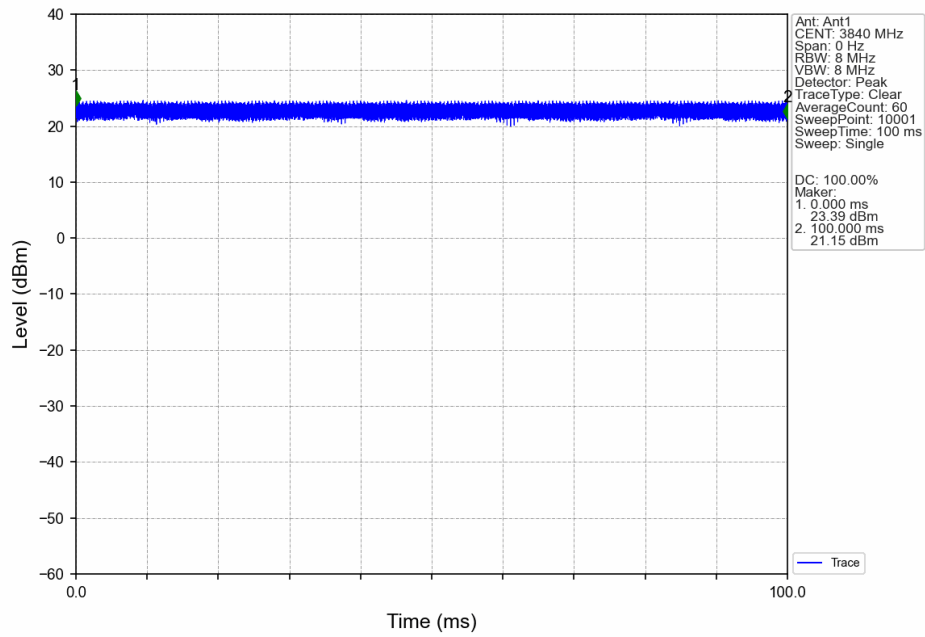
n77a_BS Type 1-C_30_Single_NTNV_CC1:40MHz_NR-FR1-TM3.1a_CC1:3840MHz_Ant1
