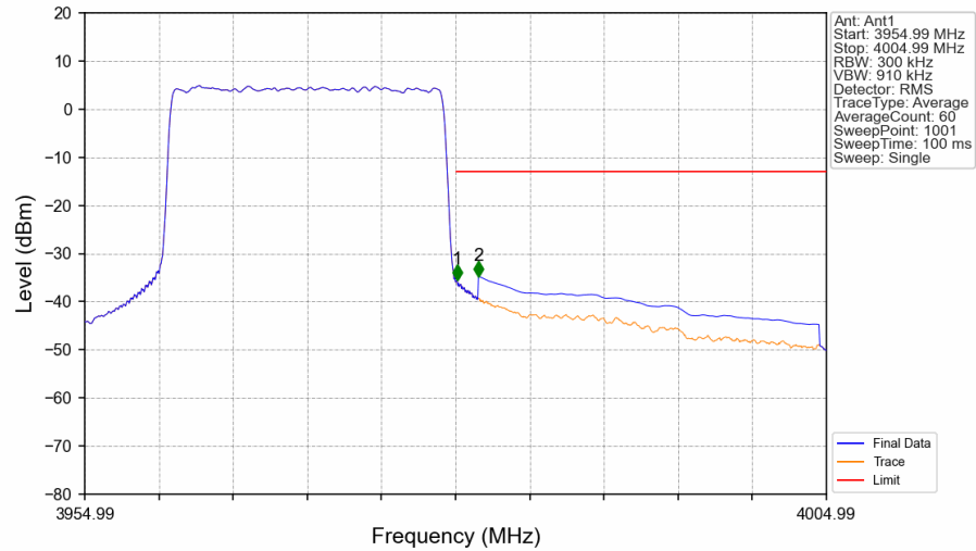
n77a_BS Type 1-C_30_Single_NTNV_CC1:20MHz_NR-FR1-TM3.1a_CC1:3969.99MHz_Ant1
