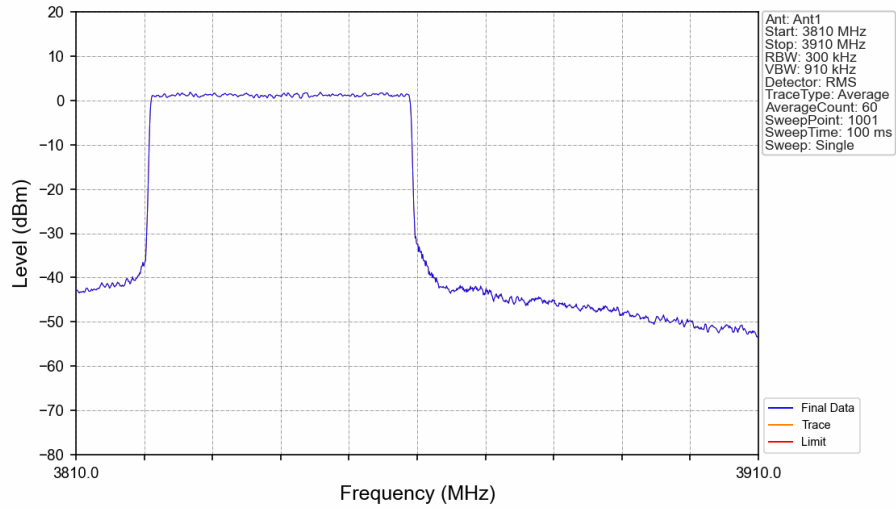
n77a_BS Type 1-C_30_Single_NTNV_CC1:40MHz_NR-FR1-TM3.1a_CC1:3840MHz_Ant1
