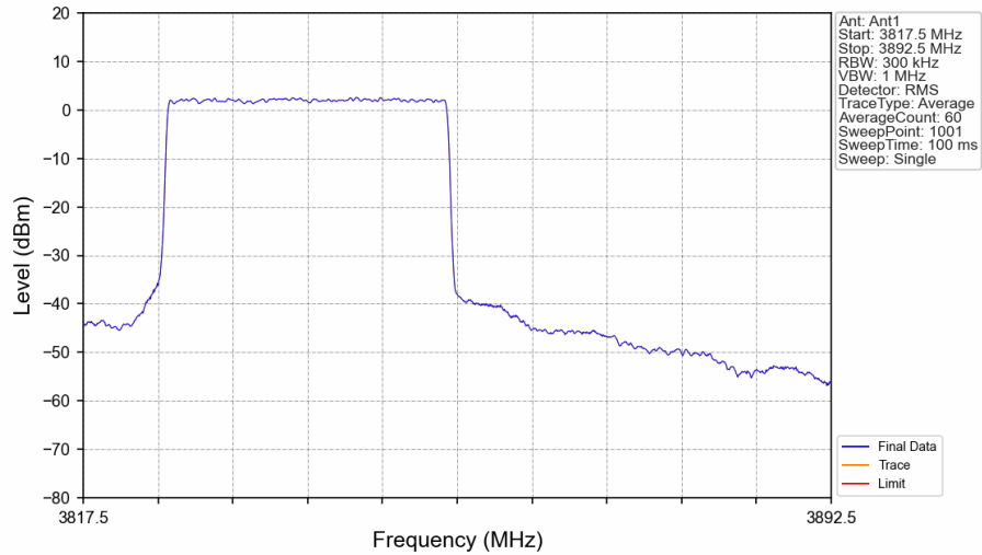
n77a_BS Type 1-C_30_Single_NTNV_CC1:30MHz_NR-FR1-TM3.1a_CC1:3840MHz_Ant1
