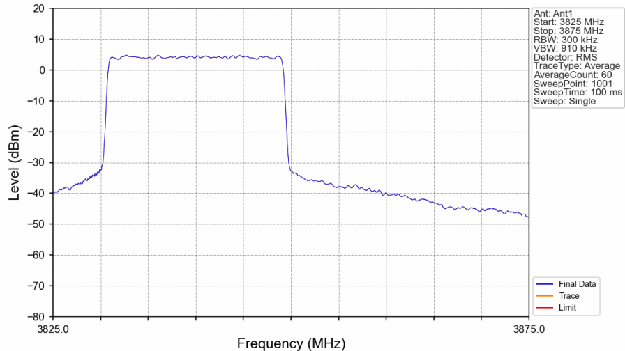
n77a_BS Type 1-C_30_Single_NTNV_CC1:20MHz_NR-FR1-TM3.1a_CC1:3840MHz_Ant1
