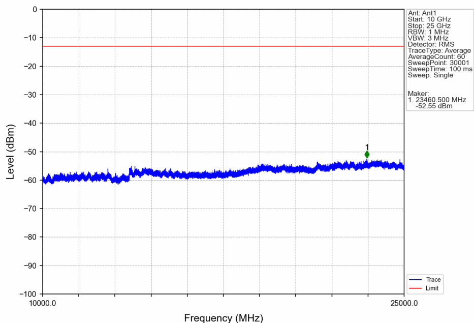
n77a_BS Type 1-C_30_Single_NTNV_CC1:20MHz_NR-FR1-TM3.1a_CC1:3969.99MHz_Ant1
