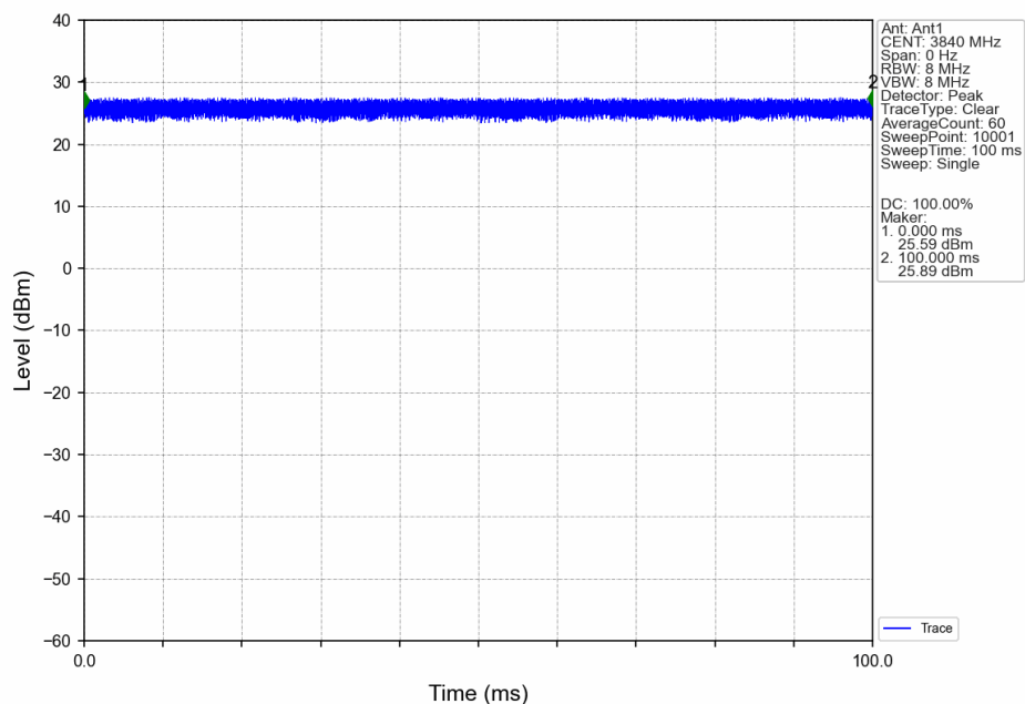
n77a_BS Type 1-C_30_Single_NTNV_CC1:20MHz_NR-FR1-TM3.1a_CC1:3840MHz_Ant1
