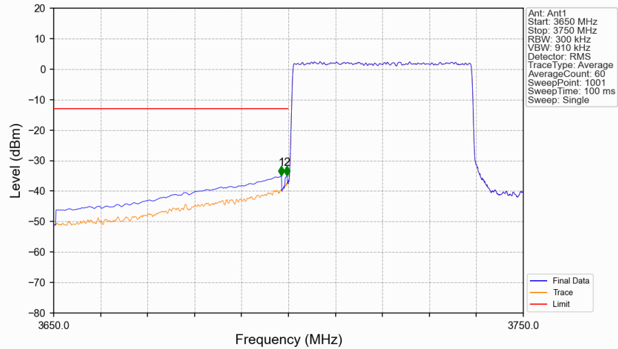
n77a_BS Type 1-C_30_Single_NTNV_CC1:40MHz_NR-FR1-TM3.1a_CC1:3720MHz_Ant1
