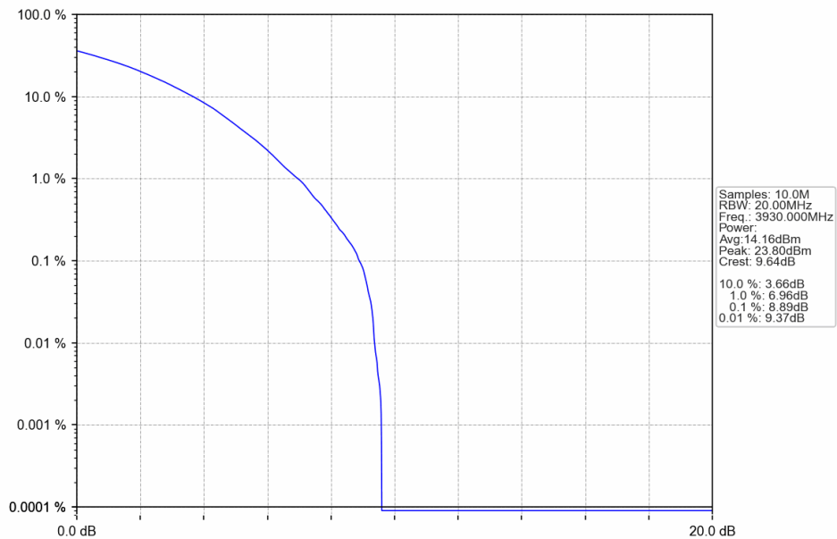
n77a_BS Type 1-C_30_Single_NTNV_CC1:100MHz_NR-FR1-TM3.1a_CC1:3930MHz_Ant1
