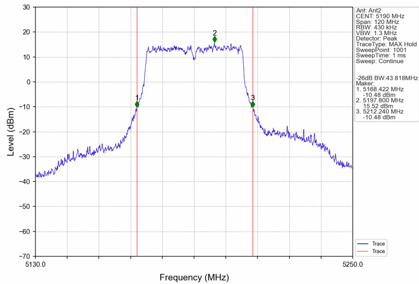
802.11ac(VHT40)_LCH_5190MHz_Ant2_NTNV
