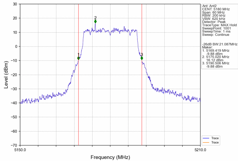
802.11ac(VHT20)_LCH_5180MHz_Ant2_NTNV
