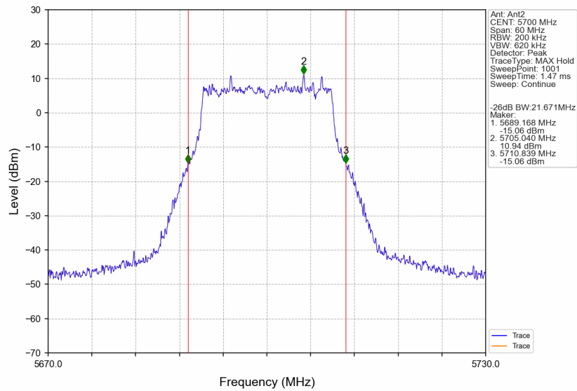
802.11ac(VHT20)_HCH_5700MHz_Ant2_NTNV
