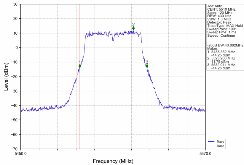
802.11ac(VHT40)_LCH_5510MHz_Ant2_NTNV
