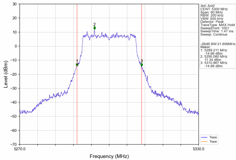
802.11ac(VHT20)_MCH_5300MHz_Ant2_NTNV
