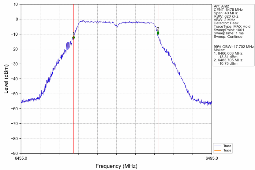
802.11ax(VHT20)_MCH_6475MHz_Ant2_NTNV
