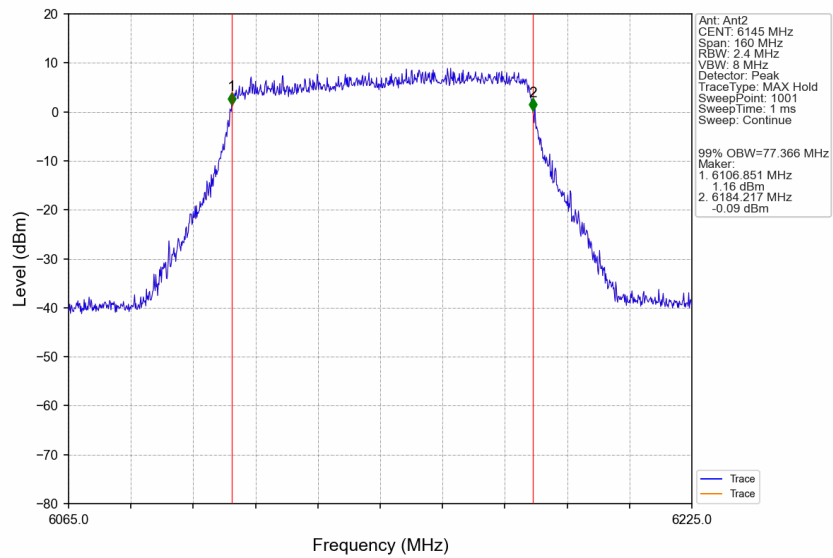
802.11ax(VHT80)_MCH_6145MHz_Ant2_NTNV
