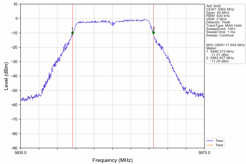
802.11ax(VHT20)_LCH_5955MHz_Ant2_NTNV
