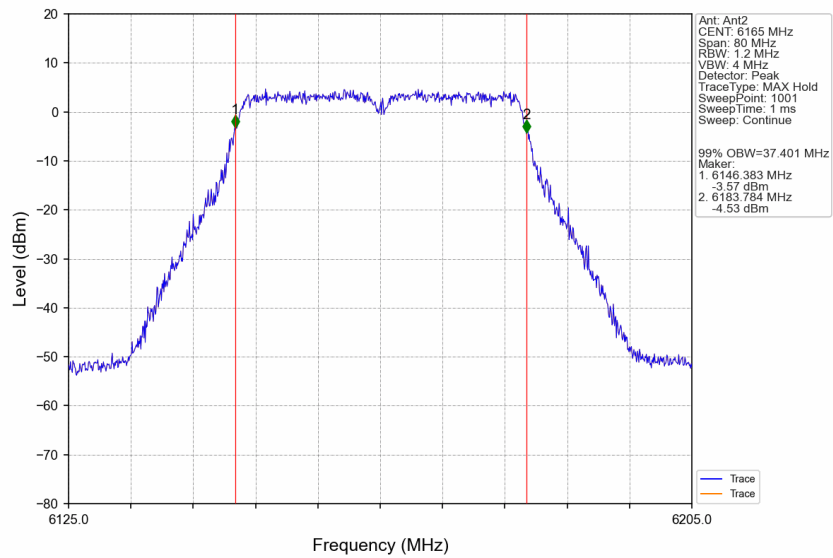
802.11ax(VHT40)_MCH_6165MHz_Ant2_NTNV
