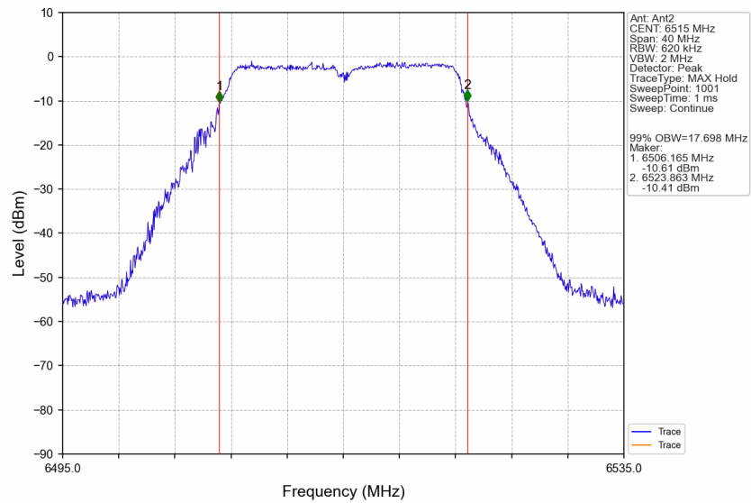
802.11ax(VHT20)_HCH_6515MHz_Ant2_NTNV
