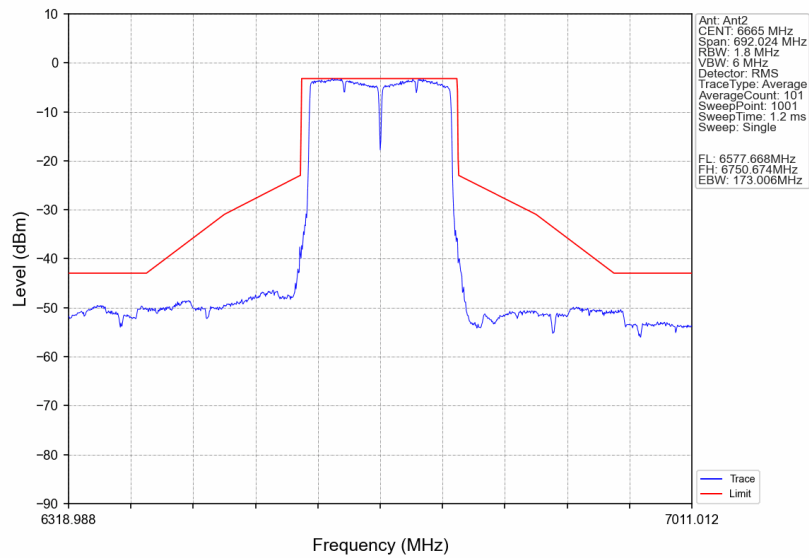
802.11ax(VHT160)_MCH_6665MHz_Ant2_NTNV
