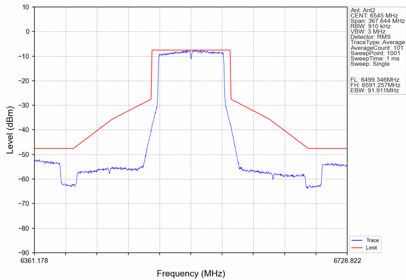
802.11ax(VHT80)_HCH_6545MHz_Ant2_NTNV
