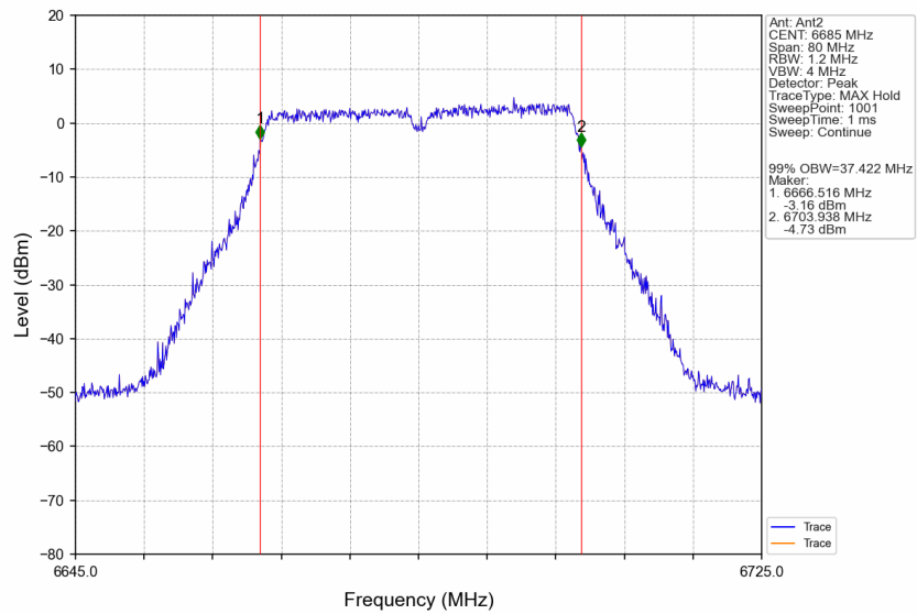
802.11ax(VHT40)_MCH_6685MHz_Ant2_NTNV
