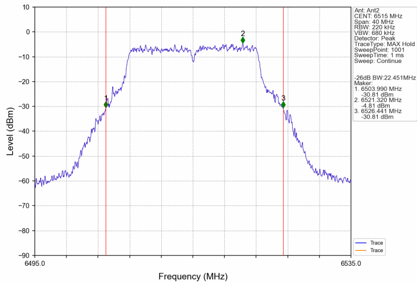
802.11ax(VHT20)_HCH_6515MHz_Ant2_NTNV
