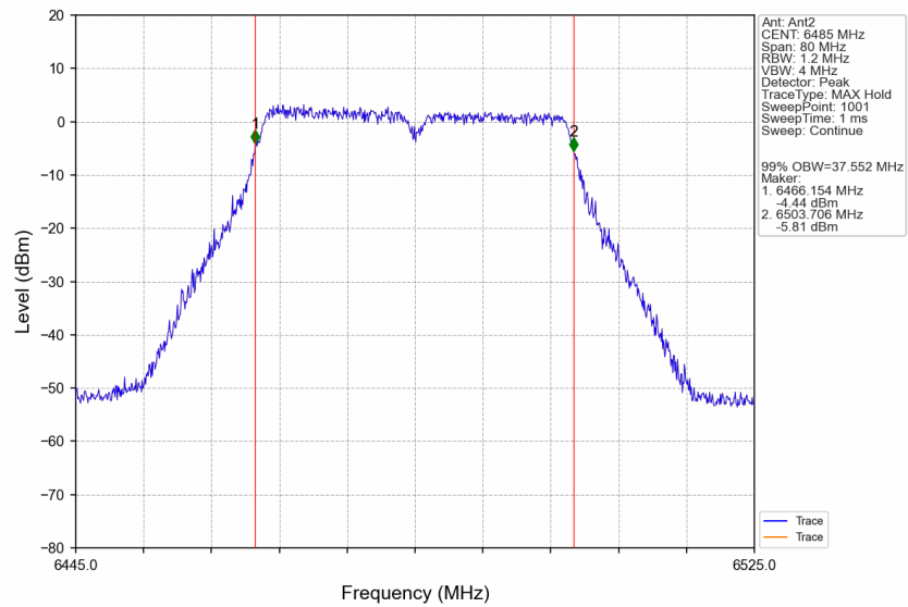
802.11ax(VHT40)_MCH_6485MHz_Ant2_NTNV
