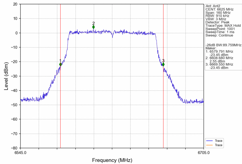
802.11ax(VHT80)_LCH_6625MHz_Ant2_NTNV
