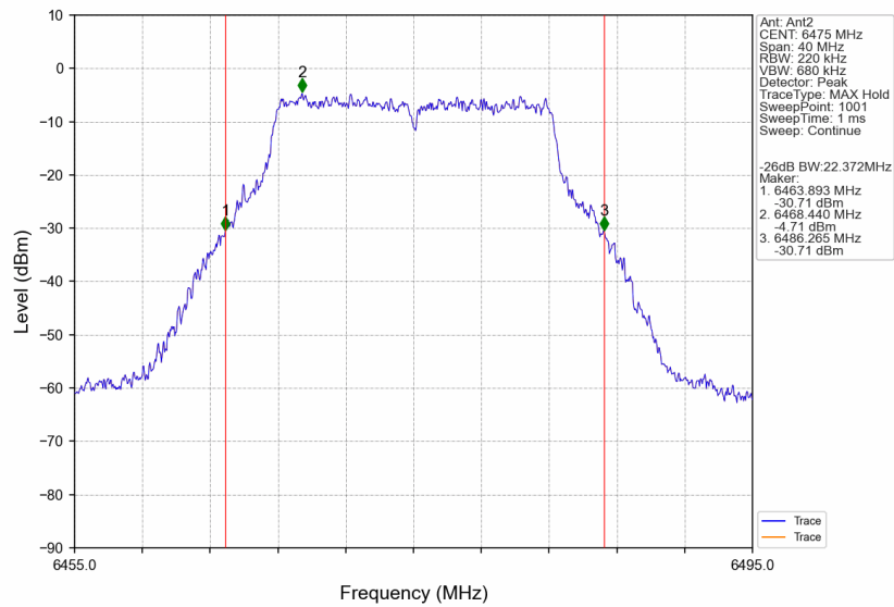
802.11ax(VHT20)_MCH_6475MHz_Ant2_NTNV
