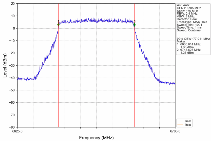
802.11ax(VHT80)_MCH_6705MHz_Ant2_NTNV
