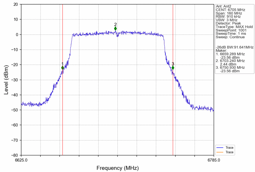
802.11ax(VHT80)_MCH_6705MHz_Ant2_NTNV
