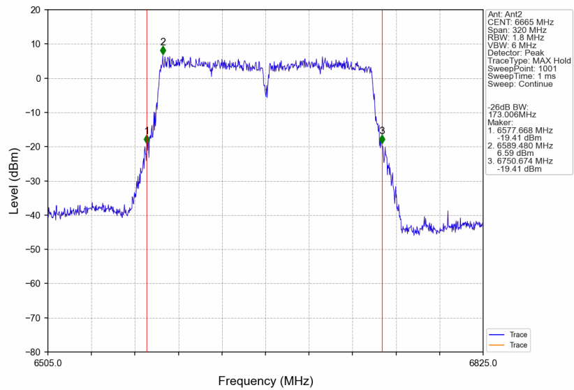
802.11ax(VHT160)_MCH_6665MHz_Ant2_NTNV
