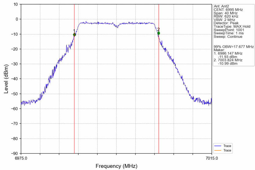
802.11ax(VHT20)_MCH_6995MHz_Ant2_NTNV
