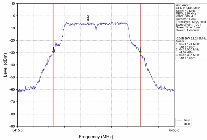
802.11ax(VHT20)_LCH_6435MHz_Ant2_NTNV
