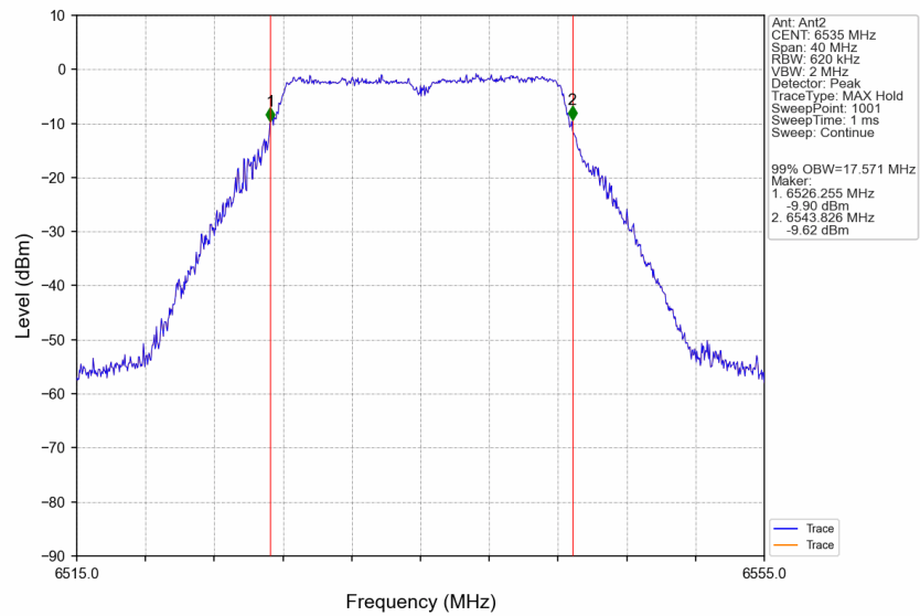
802.11ax(VHT20)_LCH_6535MHz_Ant2_NTNV
