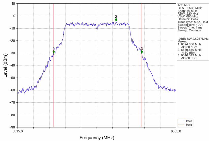
802.11ax(VHT20)_LCH_6535MHz_Ant2_NTNV
