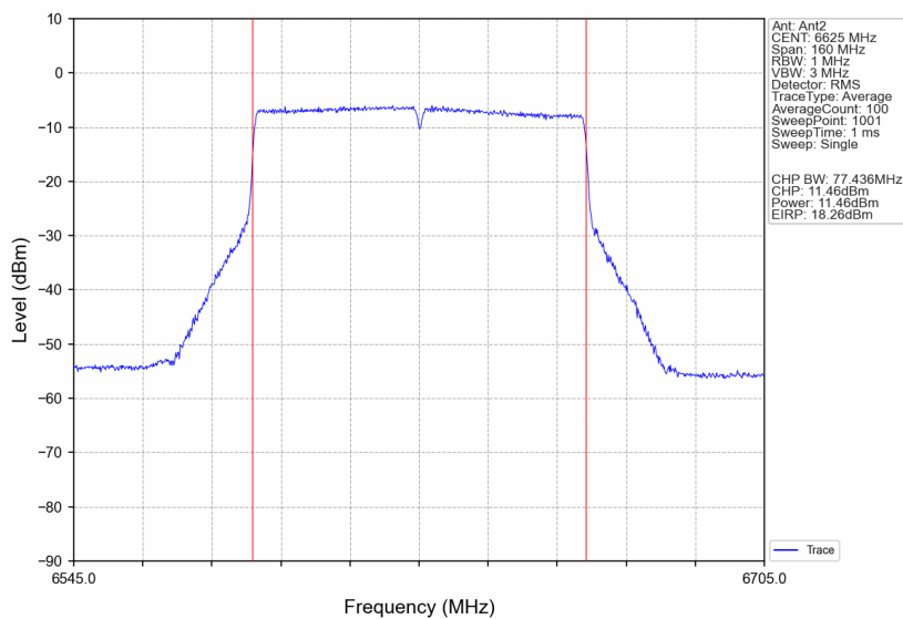
802.11ax(VHT80)_LCH_6625MHz_Ant2_NTNV
