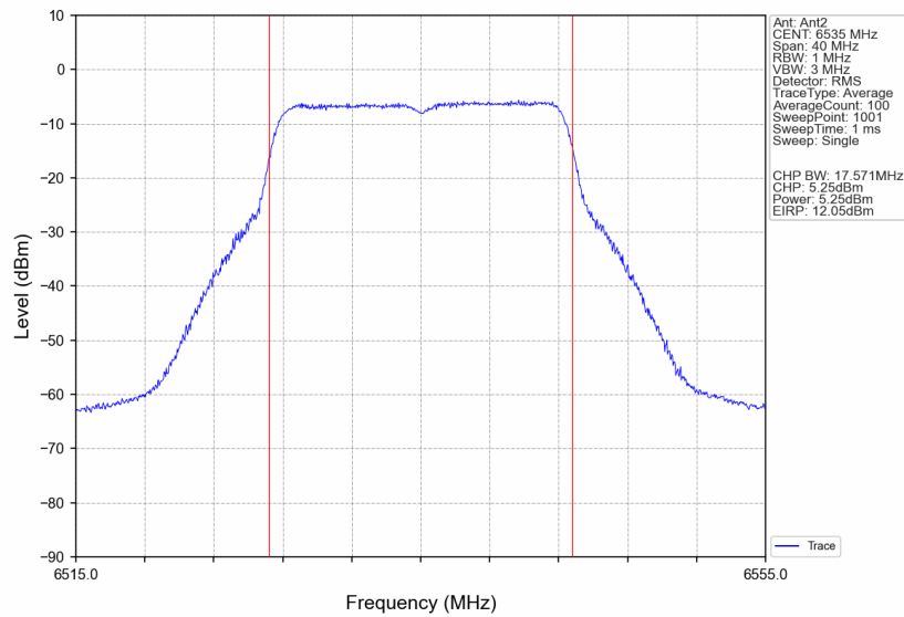
802.11ax(VHT20)_LCH_6535MHz_Ant2_NTNV
