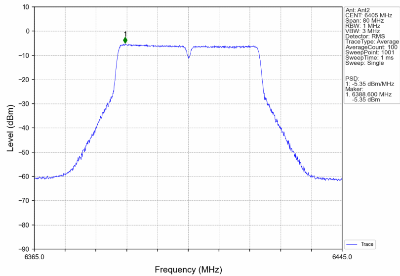
802.11ax(VHT40)_HCH_6405MHz_MIMO_NTNV
