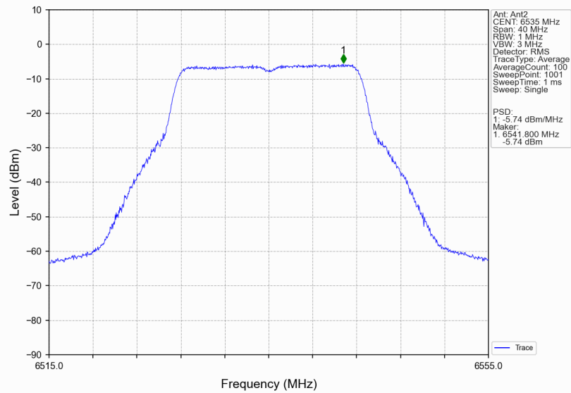
802.11ax(VHT20)_LCH_6535MHz_Ant2_NTNV
