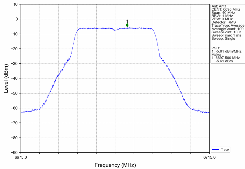
802.11ax(VHT20)_MCH_6695MHz_Ant1_NTNV
