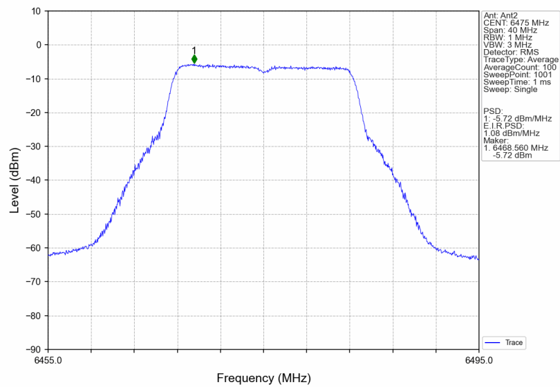
802.11ax(VHT20)_MCH_6475MHz_MIMO_NTNV
