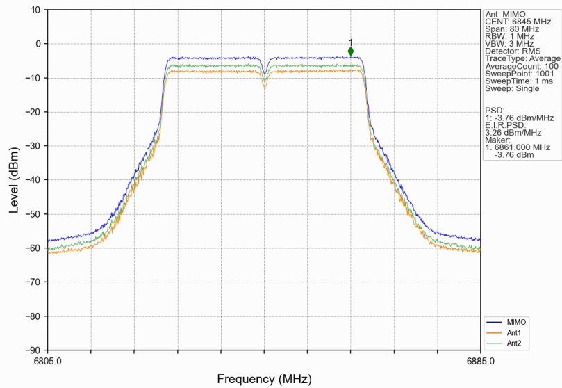
802.11ax(VHT40)_HCH_6845MHz_MIMO_NTNV
