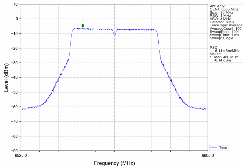
802.11ax(VHT40)_LCH_6565MHz_MIMO_NTNV
