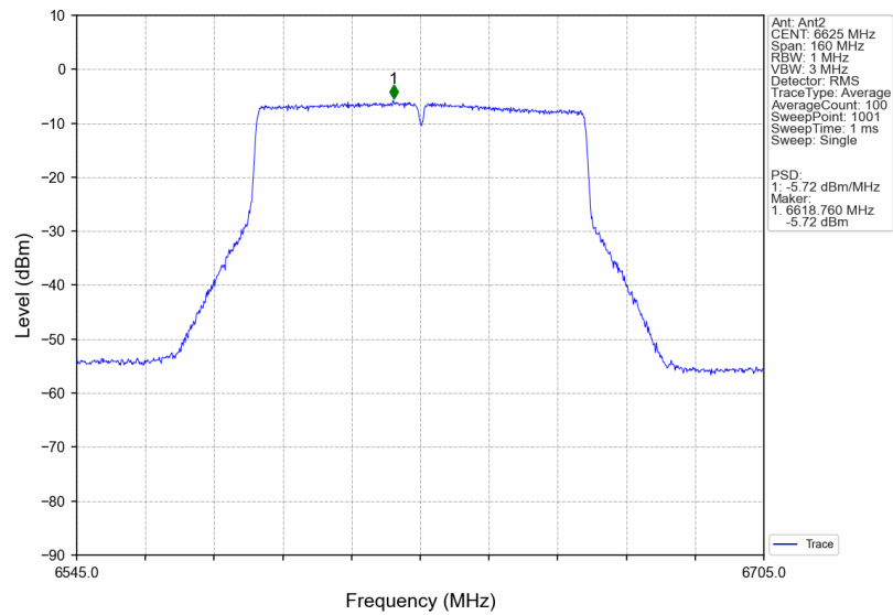
802.11ax(VHT80)_LCH_6625MHz_Ant2_NTNV
