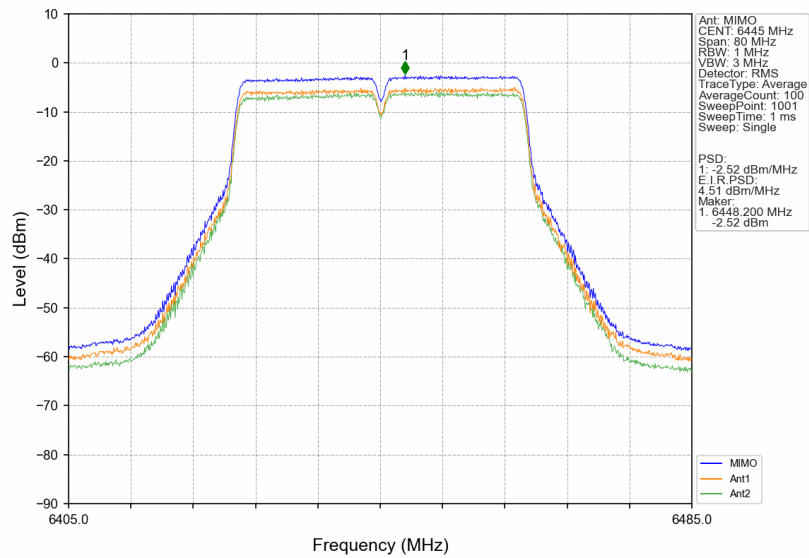
802.11ax(VHT40)_LCH_6445MHz_MIMO_NTNV
