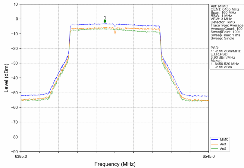
802.11ax(VHT80)_LCH_6465MHz_MIMO_NTNV
