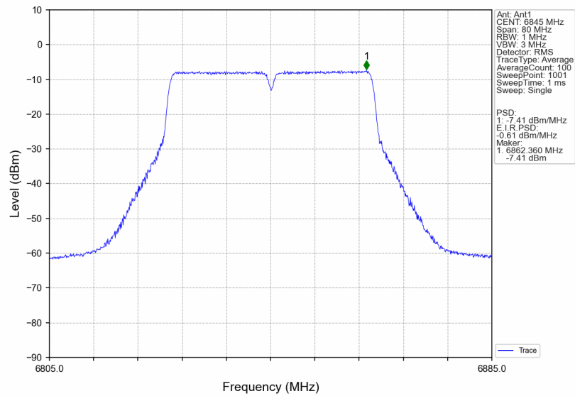
802.11ax(VHT40)_HCH_6845MHz_Ant1_NTNV
