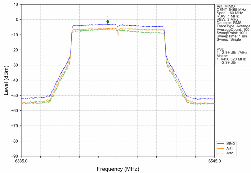
802.11ax(VHT80)_LCH_6465MHz_MIMO_NTNV
