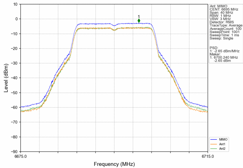
802.11ax(VHT20)_MCH_6695MHz_MIMO_NTNV
