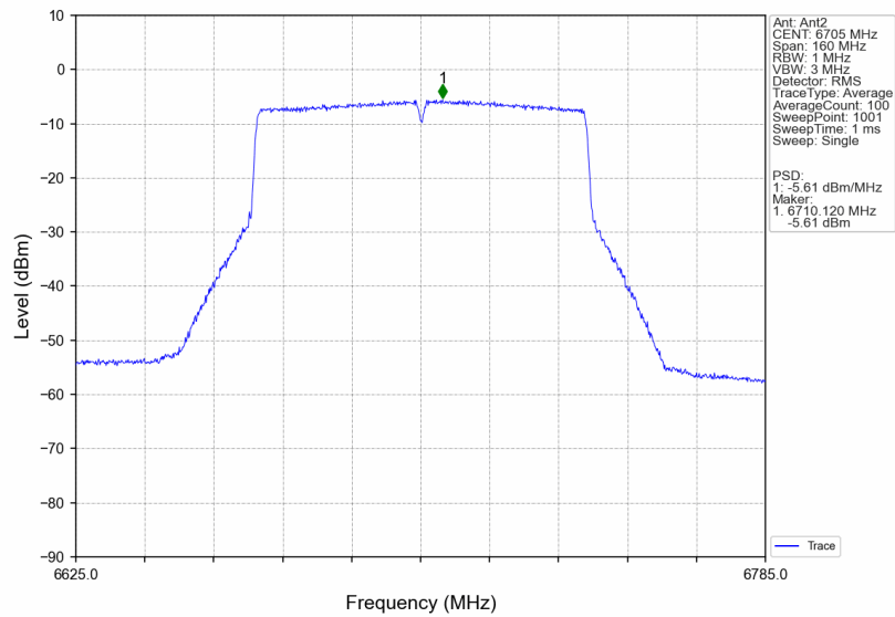
802.11ax(VHT80)_MCH_6705MHz_MIMO_NTNV
