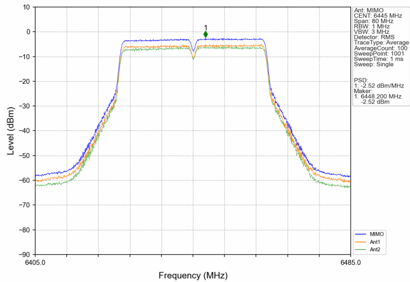
802.11ax(VHT40)_LCH_6445MHz_MIMO_NTNV
