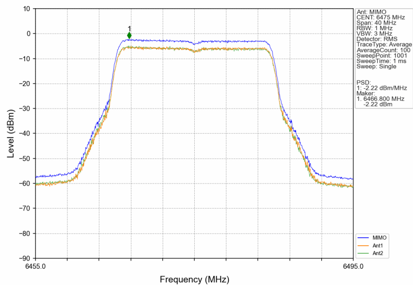
802.11be(EHT20)_MCH_6475MHz_RU242_Left_MIMO_NTNV
