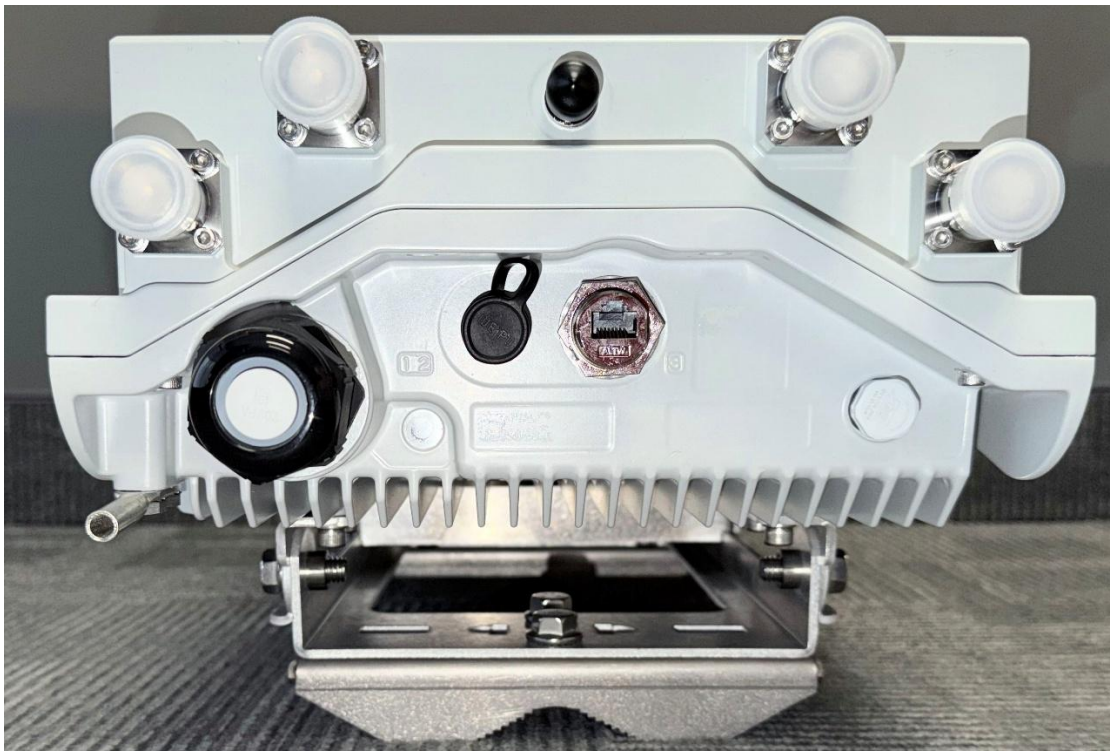
6. Bottom View (PCRF-400, PWRF-400)
