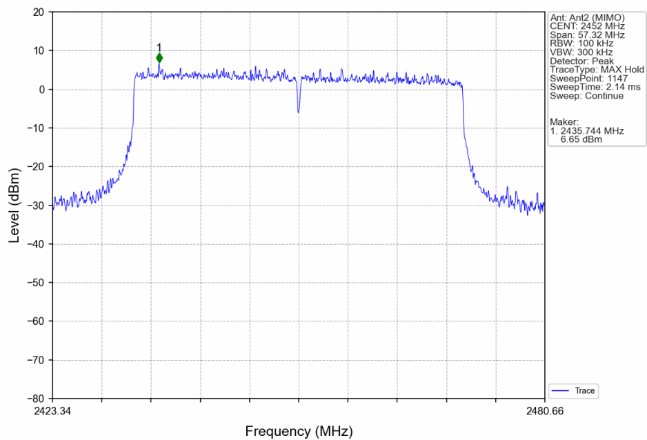
802.11ax(HEW40)_HCH_2452MHz_SU_/_Ant2 (MIMO)_NTNV
