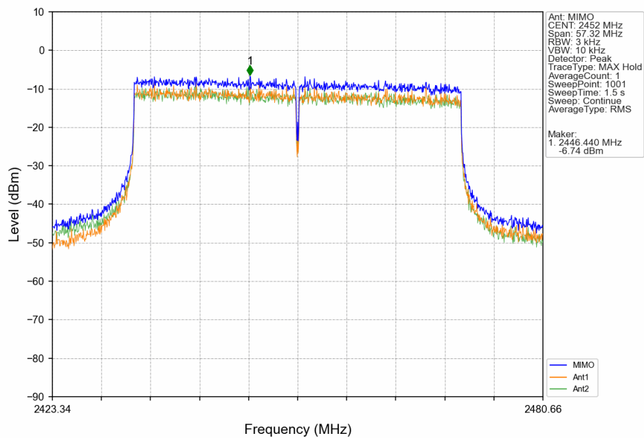
802.11ax(HEW40)_HCH_2452MHz_SU / _MIMO _NTNV
