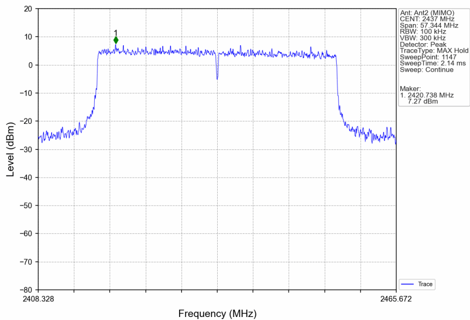
802.11ax(HEW40)_MCH_2437MHz_SU_/_Ant2 (MIMO)_NTNV
