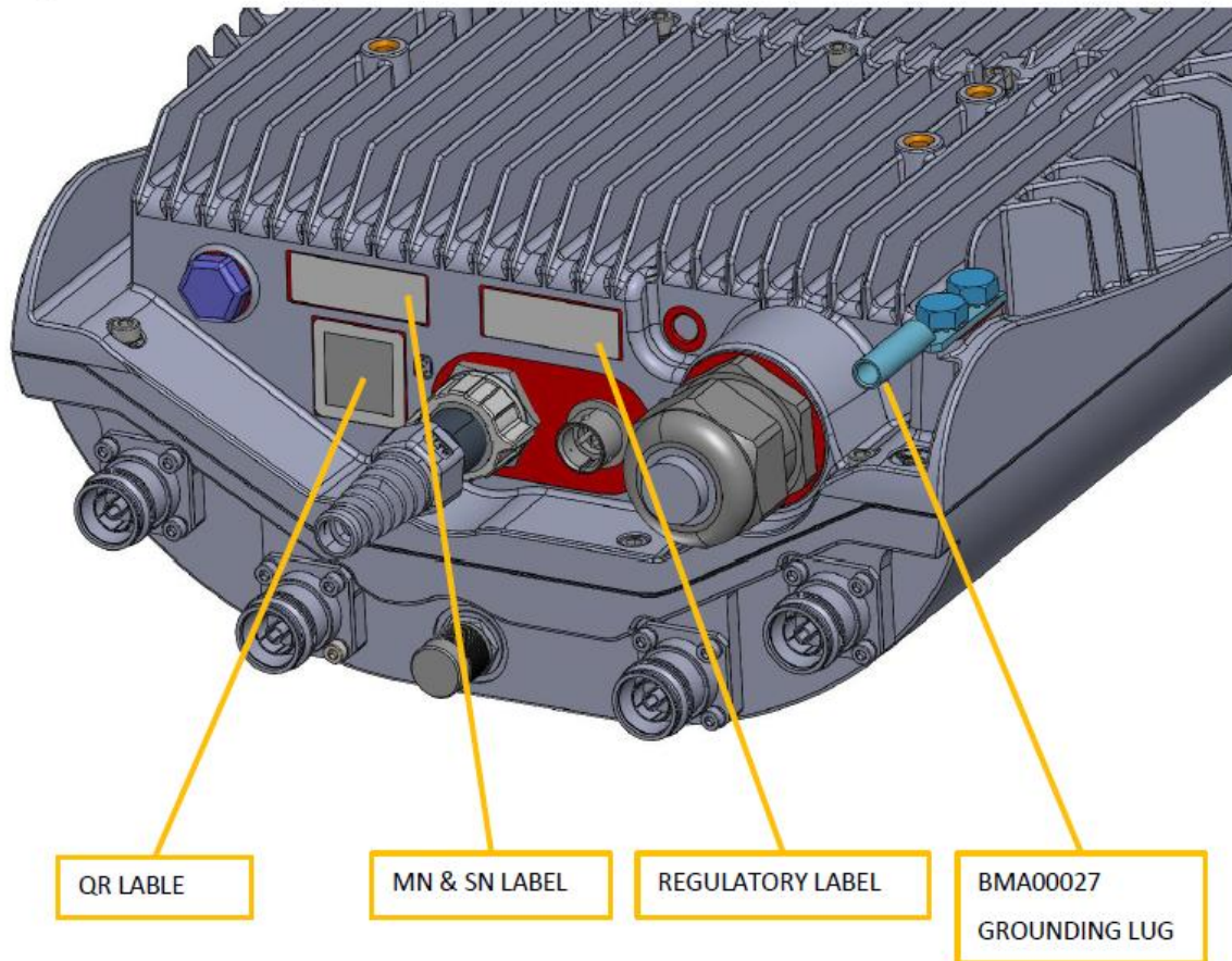
FIGURE 30: INSTALLATION OF GROUNDING LUG AND LABELS
