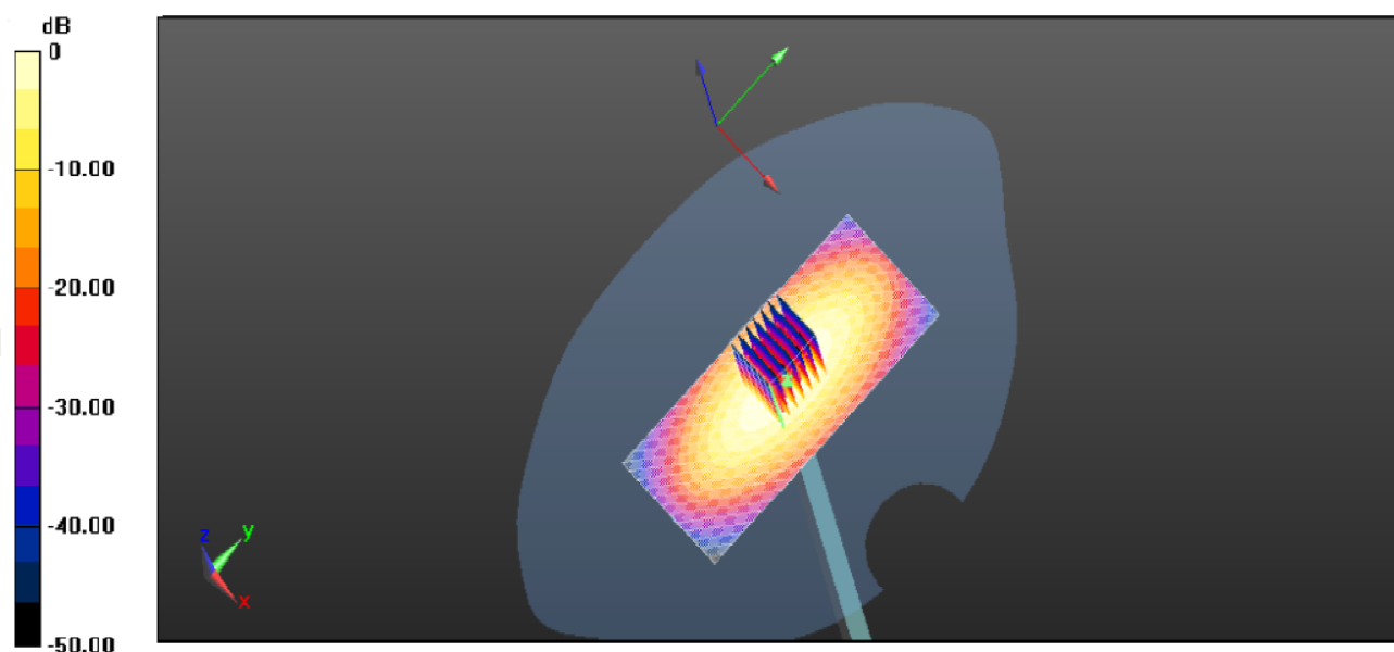
System Performance Check 1900MHz Body 250mW
