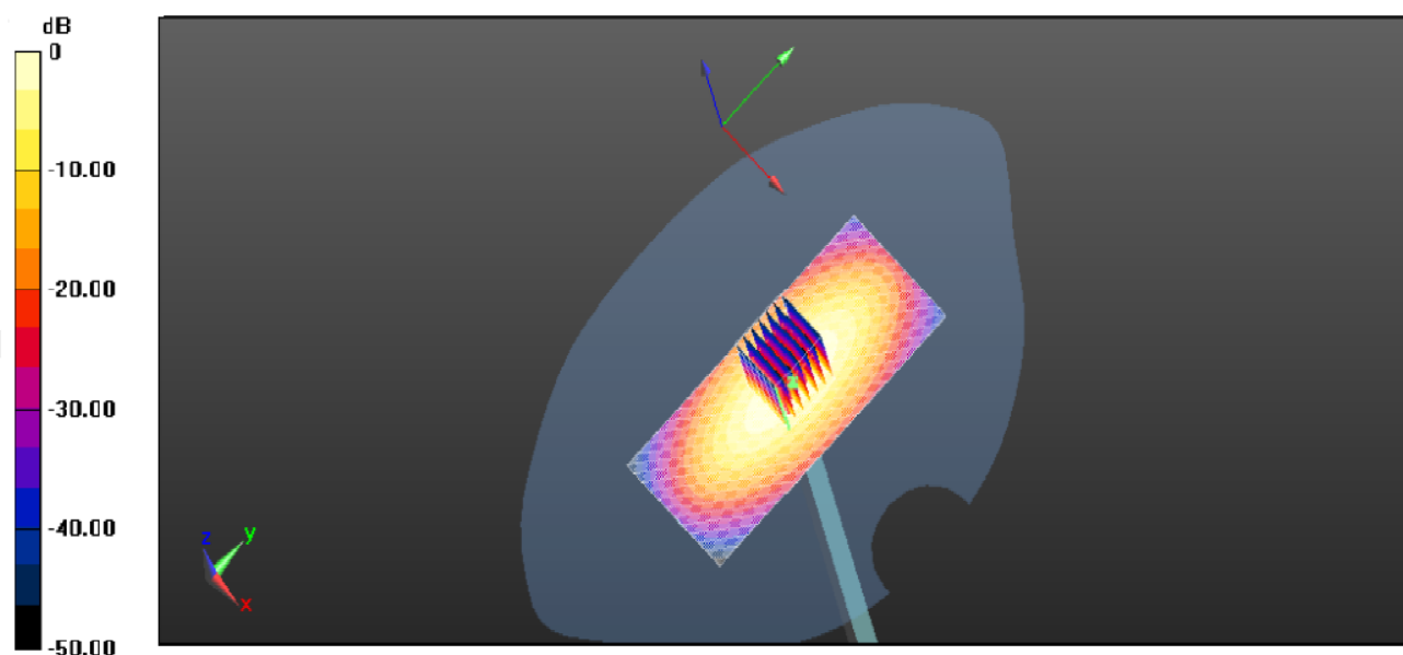
System Performance Check 835MHz Body 250mW
