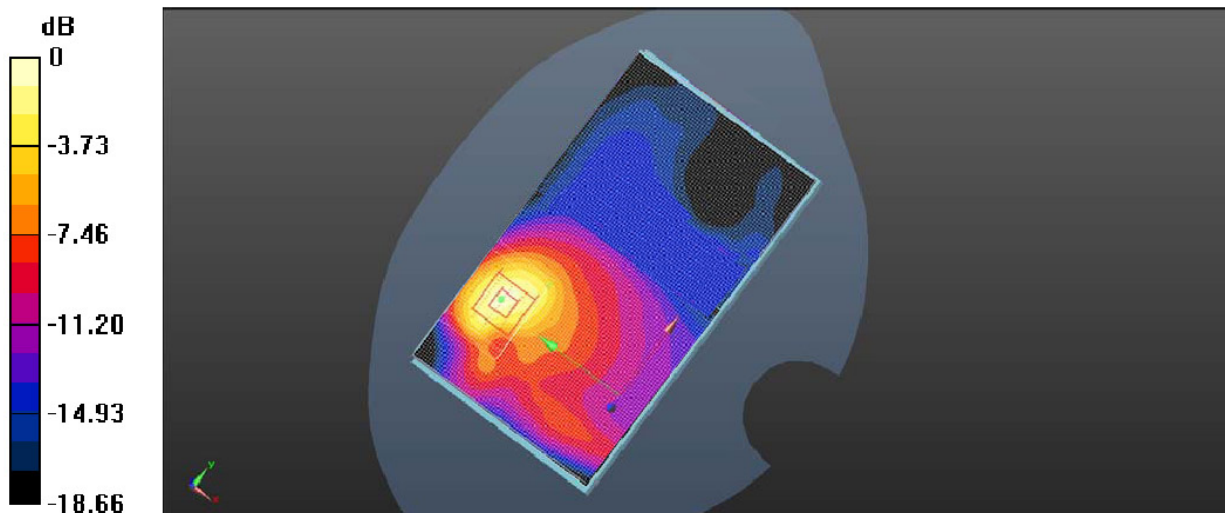
Plot 3: Body Rear Side (WCDMA Band V RMC Middle Channel)
