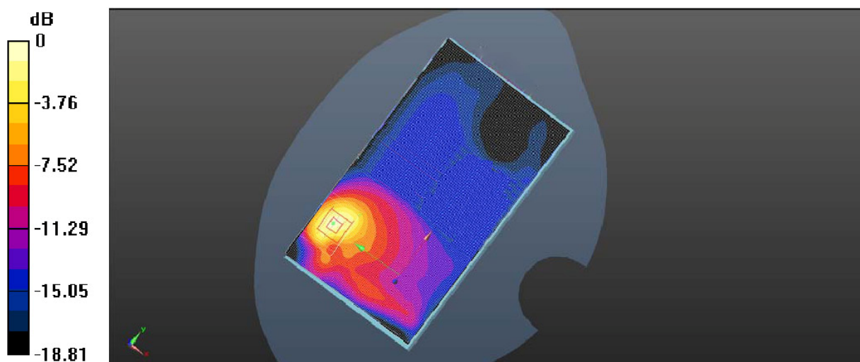
Plot 2: Body Rear Side (GSM1900 GPRS 2TS Middle Channel)
