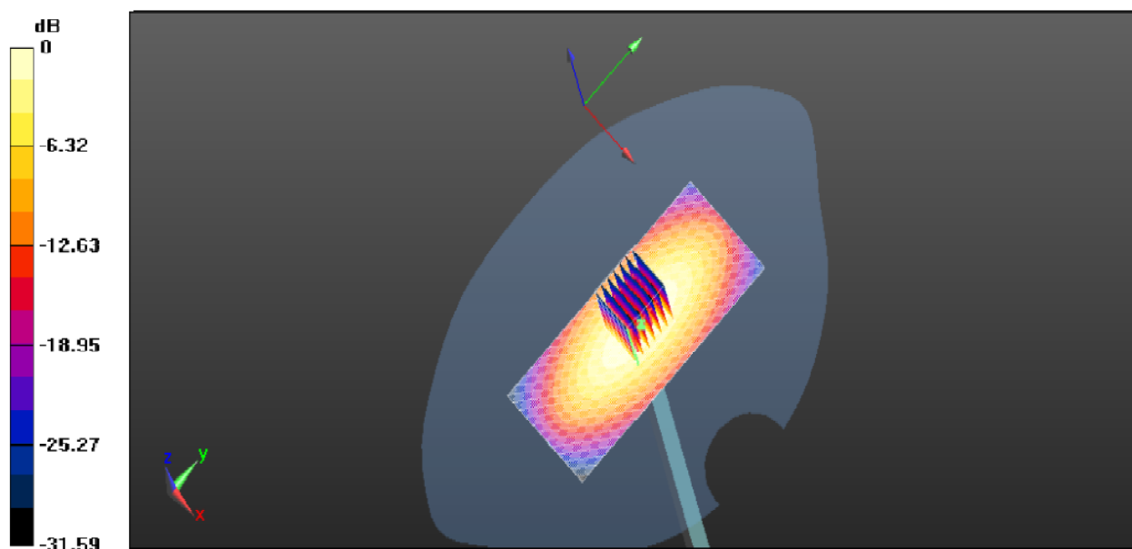
System Performance Check 2450MHz Body 250mW
