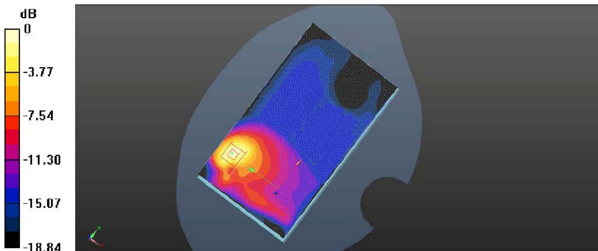
Plot 1: Body Rear Side (GSM850 GPRS 3TS Middle Channel)
