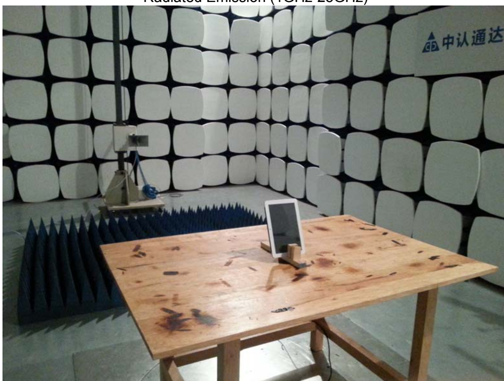
Radiated Emission (1GHz-25GHz)
