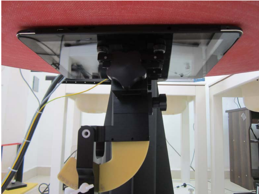
0mm Body-worn Rear Setup Photo
