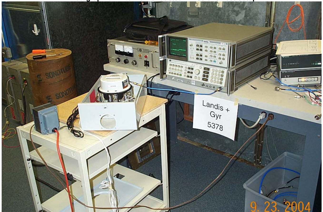
Photograph of Antenna Conducted Emissions Test Setup
