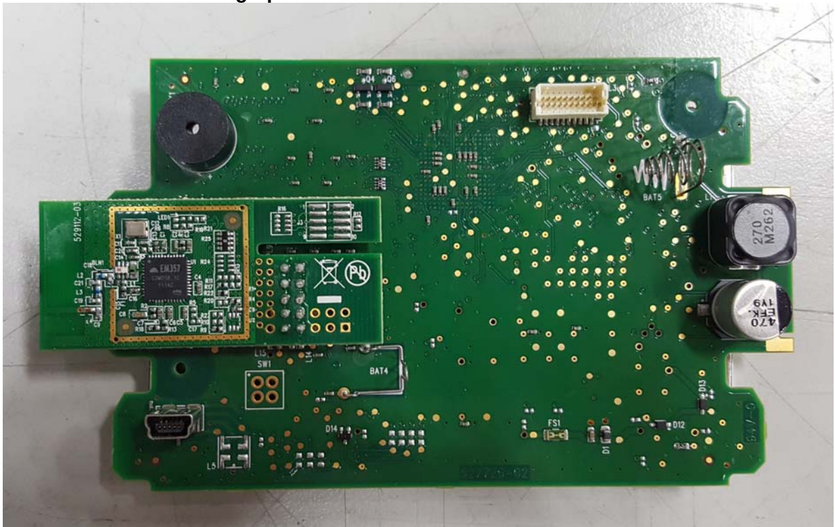
Photograph of Main Board with RF board installed
