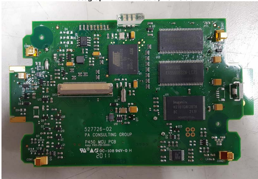
Photograph of Main Board; LCD side
