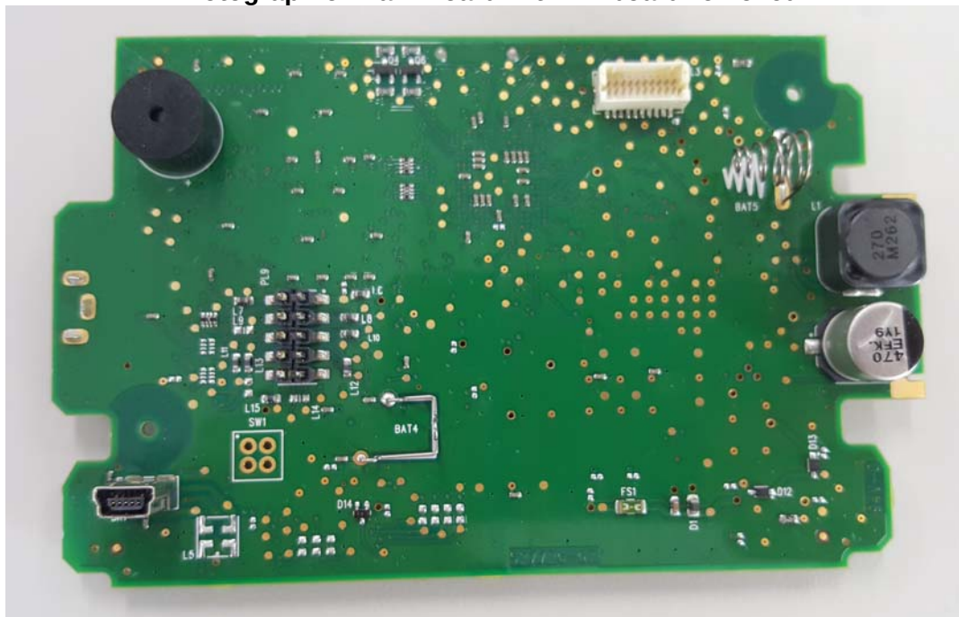
Photograph of Main Board with RF board removed
