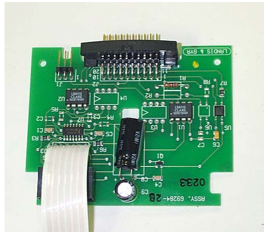
Component side
