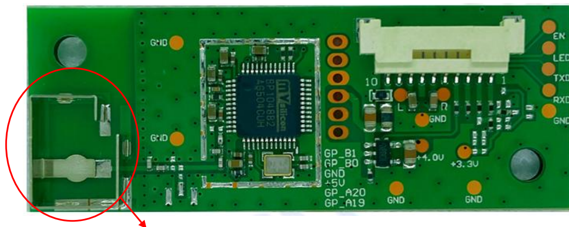
Figure 3 Inside of the EUT
