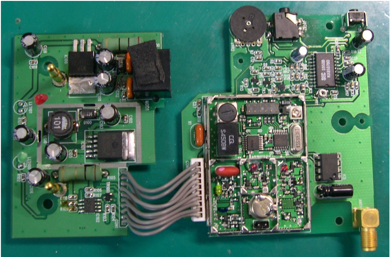
<Photograph 3: BASE, RF module shielding cover removed >
