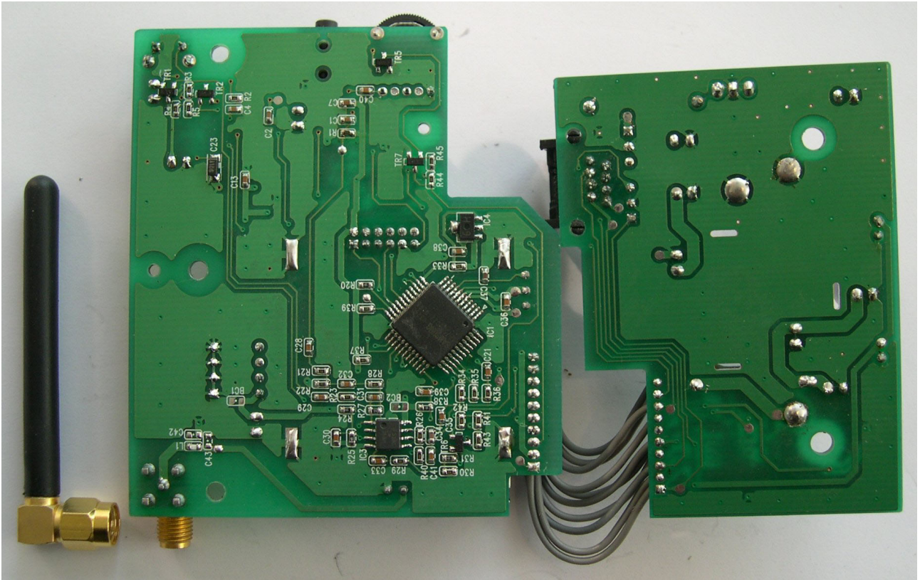
<Photograph 4: BASE - Rear View >
