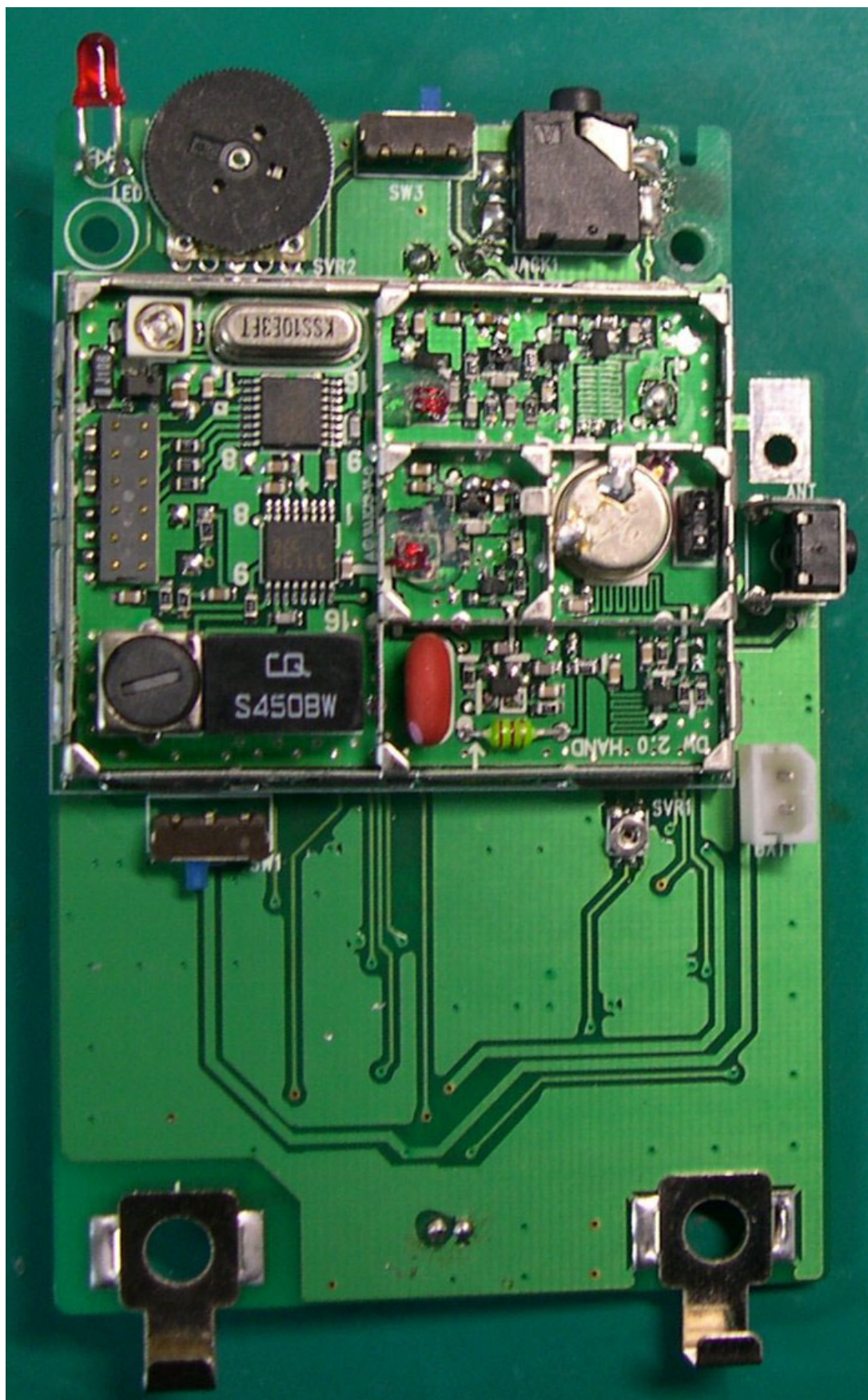
<Photograph 3: HANDSET, RF module shielding cover removed >
