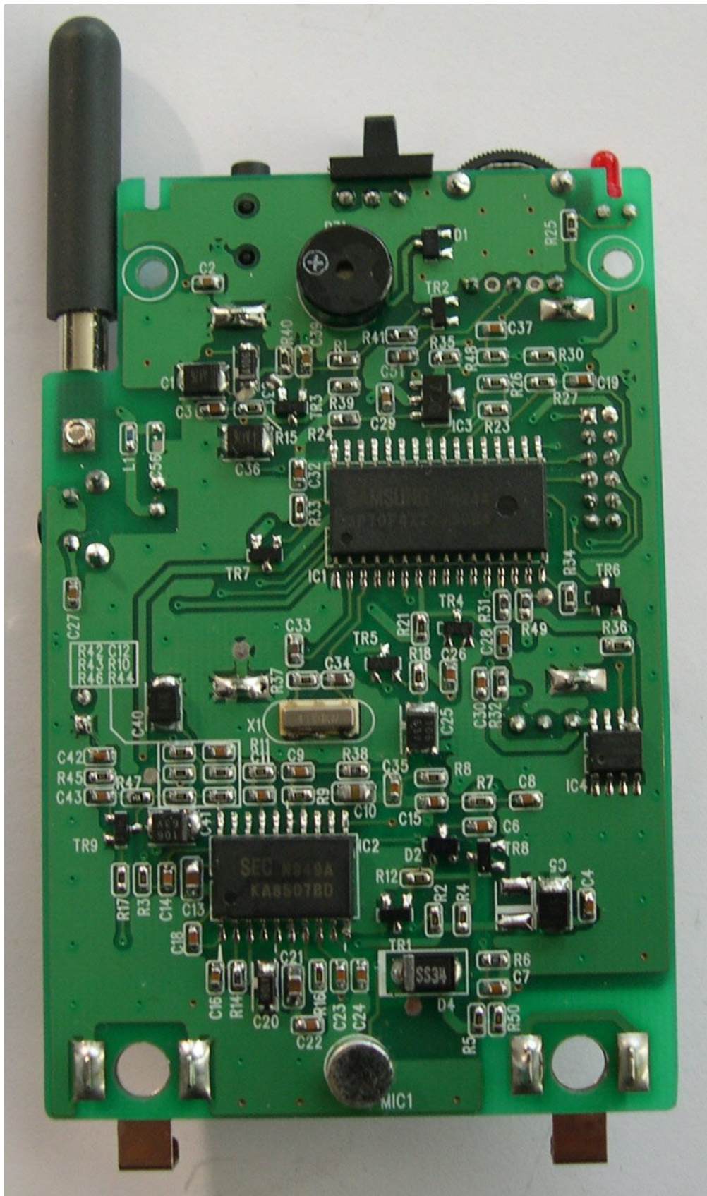
<Photograph 4: HANDSET - Rear View >
